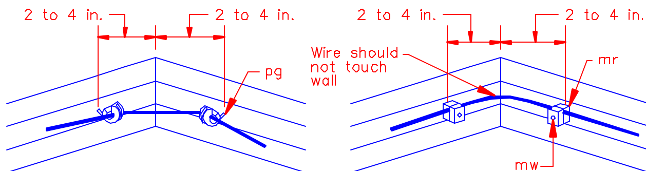
INSIDE CORNER
