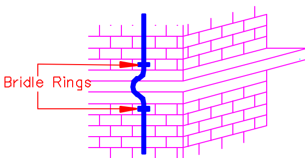
SKETCH F: MASONRY BUILDING PROJECTIONS
