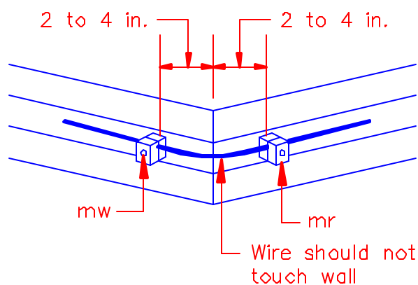
OUTSIDE CORNER
