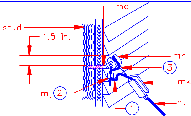
VERTICAL BUILDING RUN(Angle Screw)
