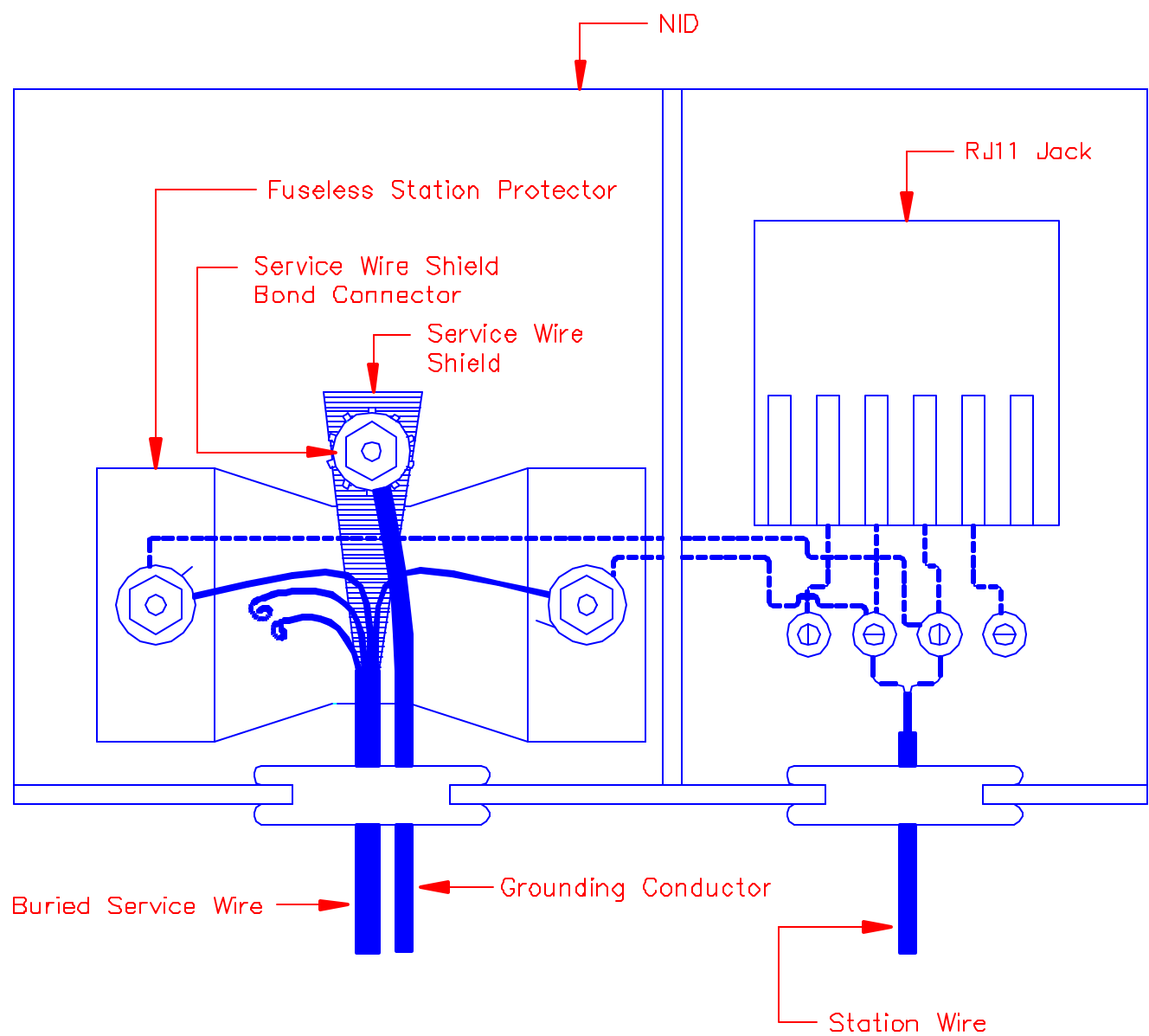
FIGURE 19 NID TERMINATIONS
