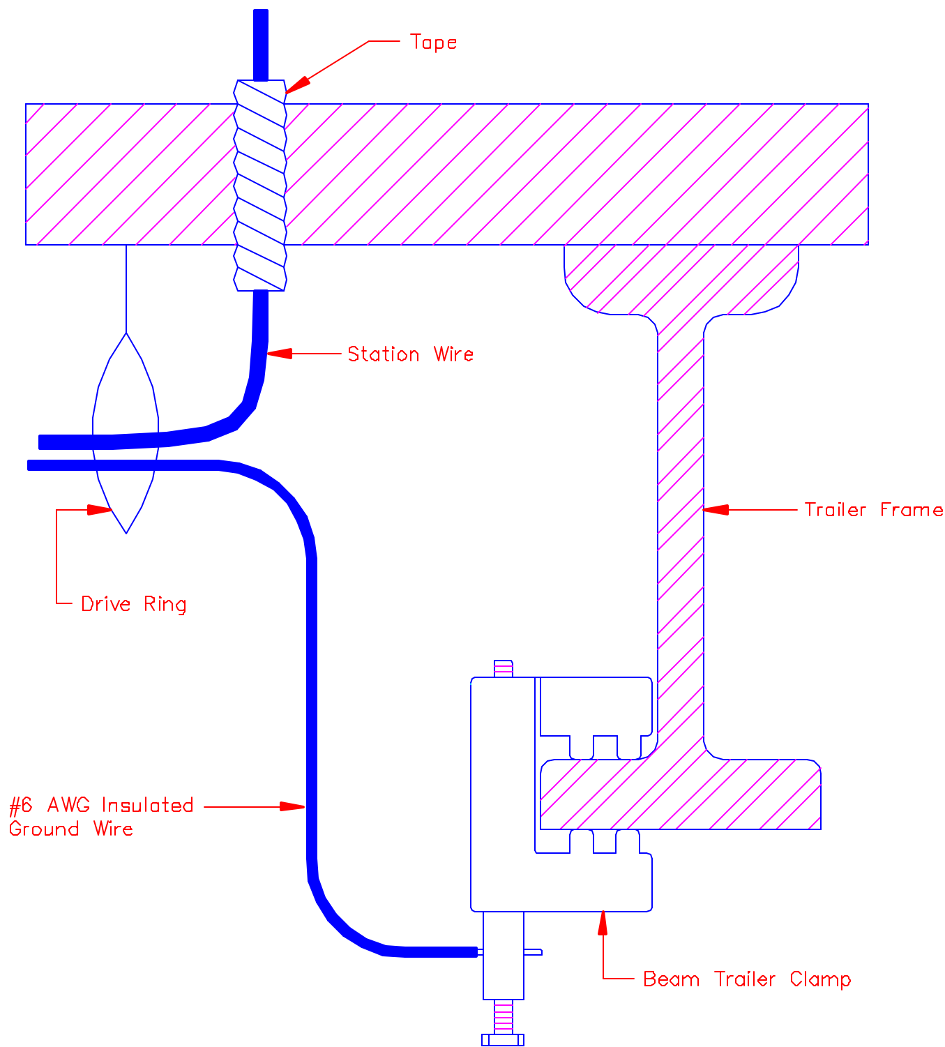
FIGURE 20 MOBILE HOME INSTALLATION
