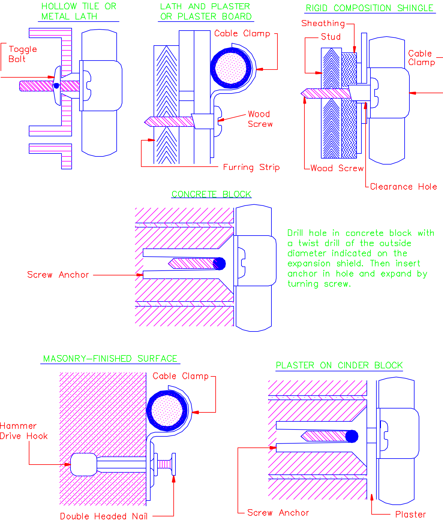
FIGURE 2 CABLE ATTACHMENT DEVICES
