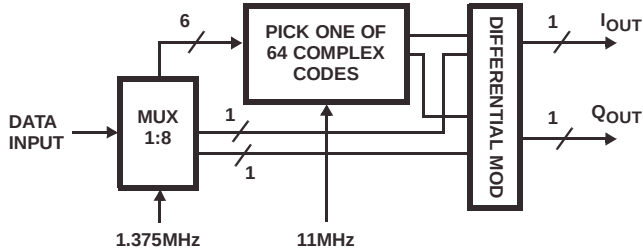
FIGURE 1. BLOCK DIAGRAM OF HFA3861A MODULATOR CIRCUIT
