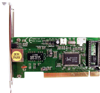
Figura 2.1 Tarjeta Ethernet
