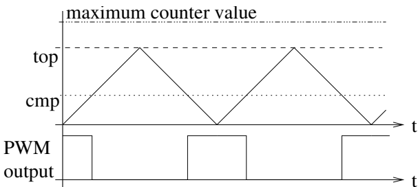
Slika : PWM signal generated by an up-down-counter.
