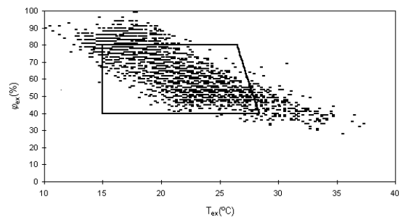
Fig. 3 –Exterior thermal environment in summer period.
