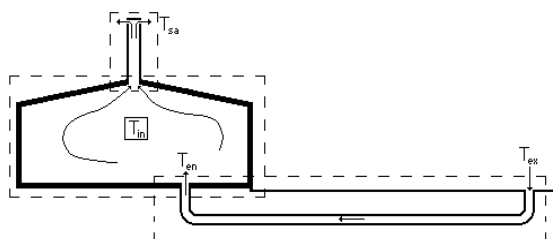
Fig. 1 – Building, solar chimney and buried pipes.
