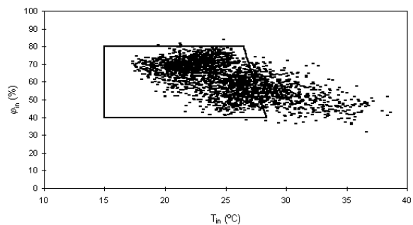
Fig. 4 - Thermal environment , inside the livestock building without solar chimney and buried pipes, in summer period.
