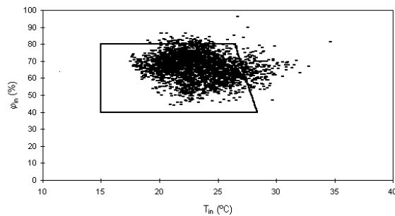
Fig. 5 - Thermal environment, inside the livestock building with solar chimney and buried pipes, in summer period.
