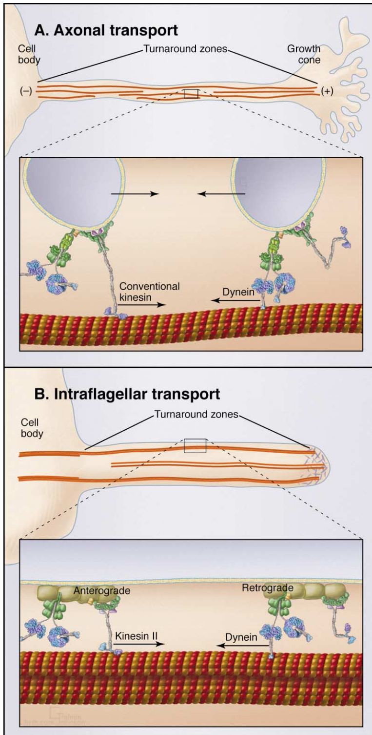
Figure 2. Coordination of Opposite Polarity Motors in Axonal and Intraflagellar Transport
