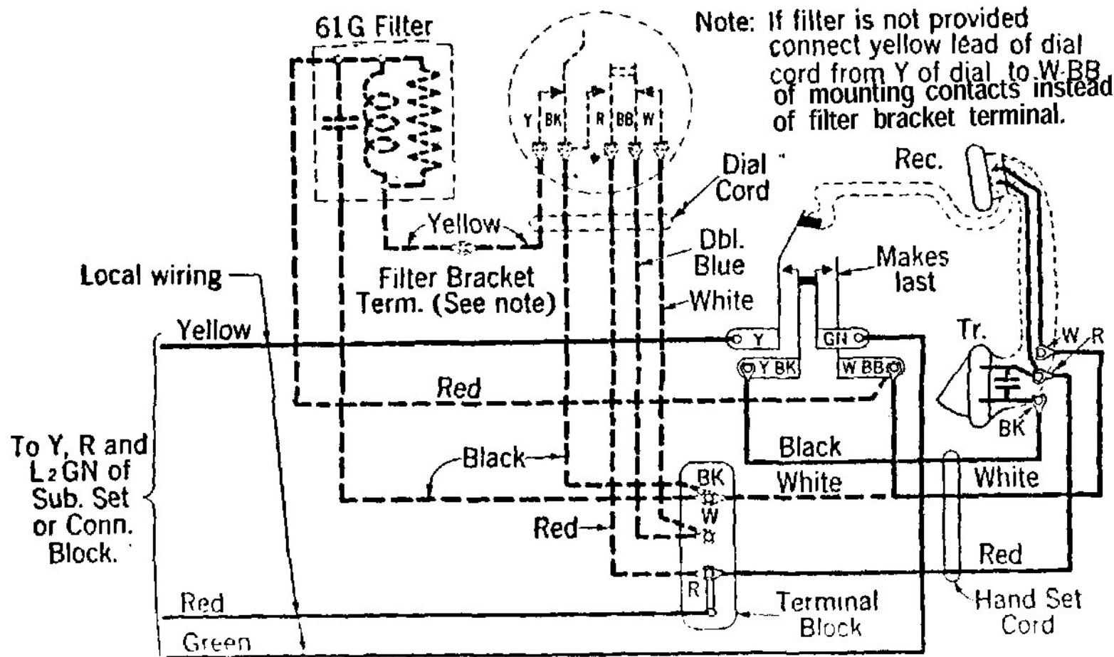
Fig. 2-201 Type Sidetone Hand Telephone Sets
