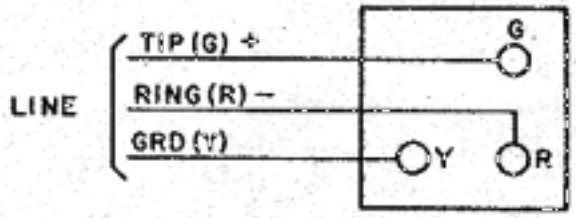
STANDARD CONNECTOR BLOCK WIRING
