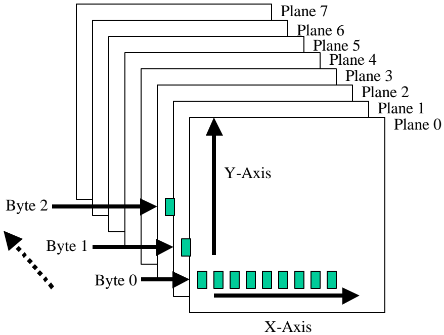
Interleaved Organization
