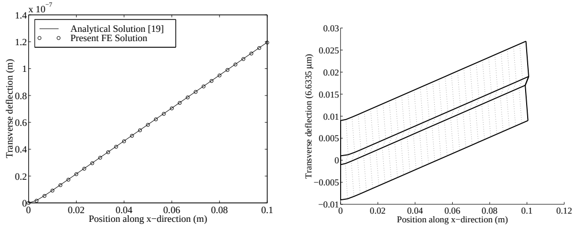
Figure 4: a) Transverse displacement of the beam. b) Deformed configuration of the beam.
