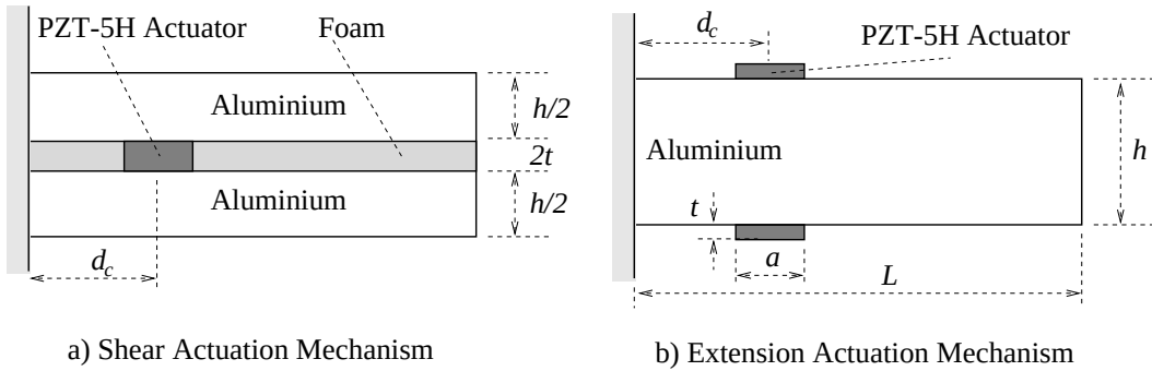
Figure 3: Cantilever sandwich beam, shear and extension actuation mechanisms.
