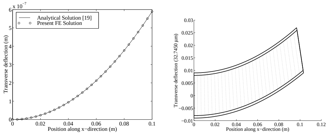
Figure 5: a) Transverse displacement of the beam. b) Deformed configuration of the beam.
