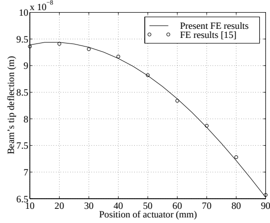
Figure 6: Beam's tip transverse displacement for several actuator's positions.
