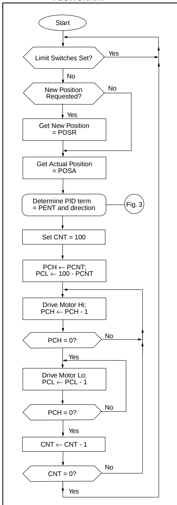
FIGURE 2: PROGRAM FLOWCHART
