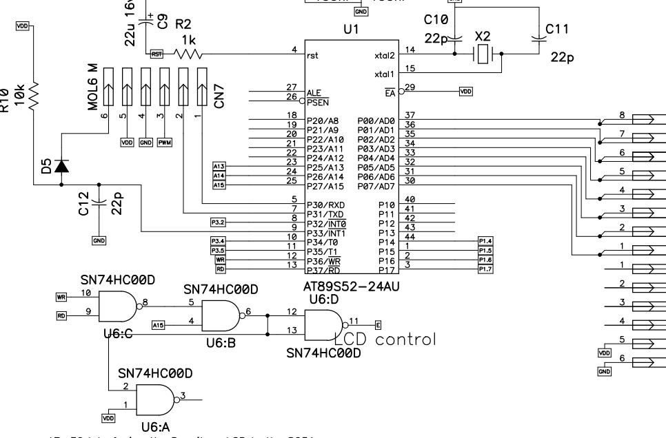
AB-39 Interfacing the Densitron LCD to the 8051 from Intel
