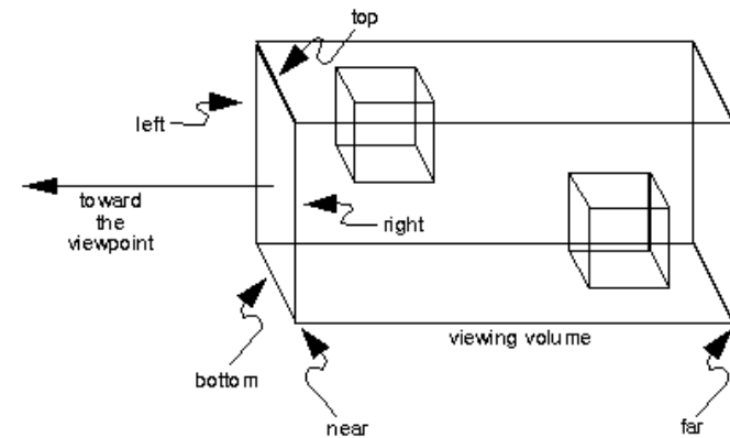
Figure 3-13 The Orthographic Viewing Volume
