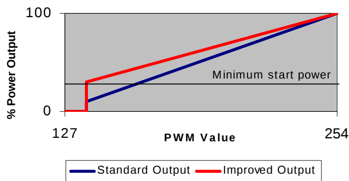
Figure 2: Example of improved output from speed controller (forward only shown)
