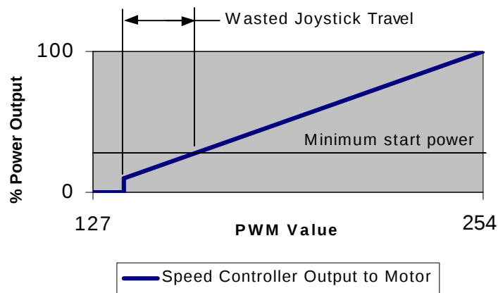
Figure 2: Example of improved output from speed controller (forward only shown)
