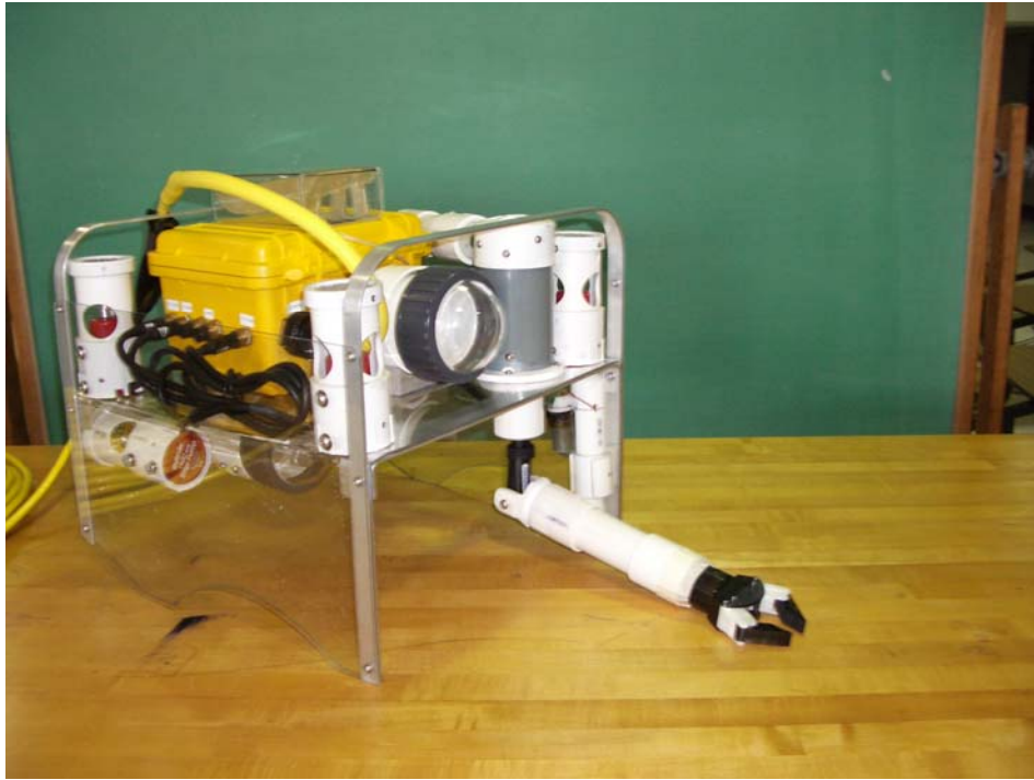
Argo Navis Front View with Arm Extended
