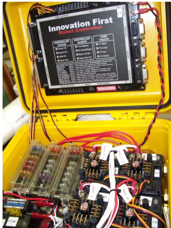
Argo Navis ROV Control Box
