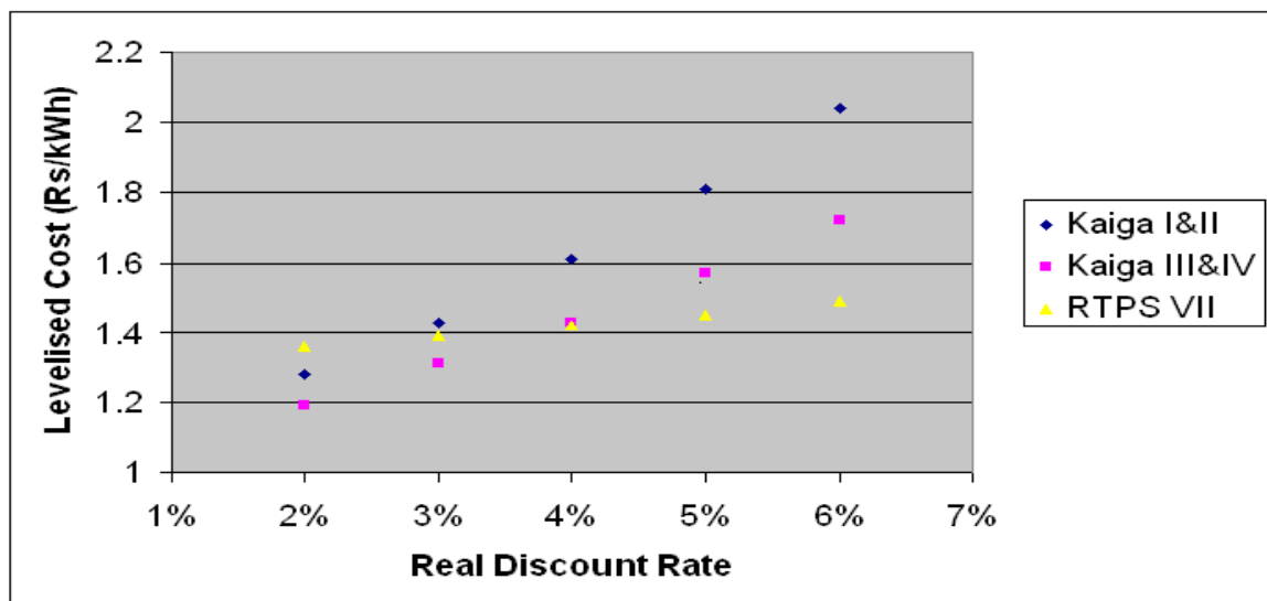
Figure 1: Levelised cost (the bare generation cost which does not include other components of electricity tariff like interest payments and transmission and distribution charges) of Kaiga I&II (operating reactors), Kaiga III&IV (reactors under construction; projected costs), and RTPS VII (operating thermal plant) as a function of real discount rate (a measure of the value of capital after taking out the effects of inflation).
