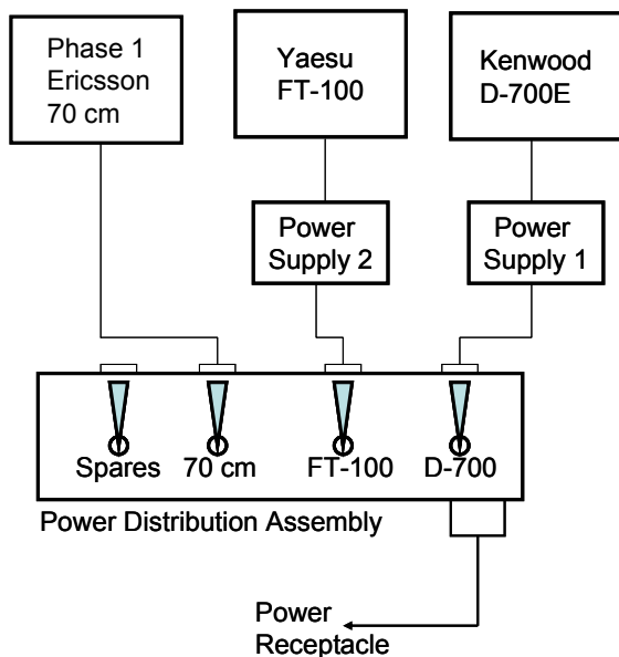
Power Distribution Schematic Figure 11
