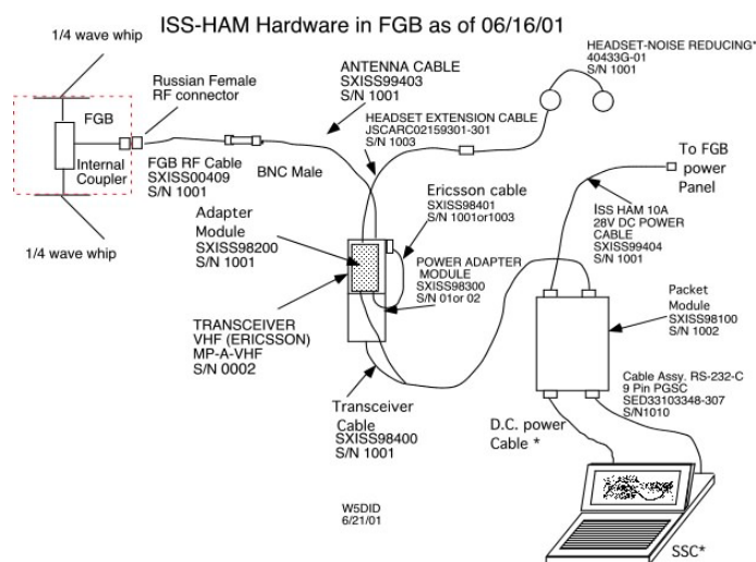
ISS Ham Phase 1 System in the FGB Figure 3
