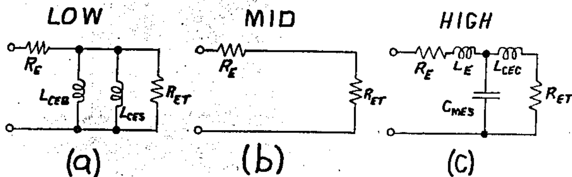
Fig. 4. Reductions of the horn-driver system simplified electrical equivalent circuit of Fig. 2 in each frequency band indicated in Fig. 3. It is assumed that f_c \ll f_{LC} as in Fig. 3.
