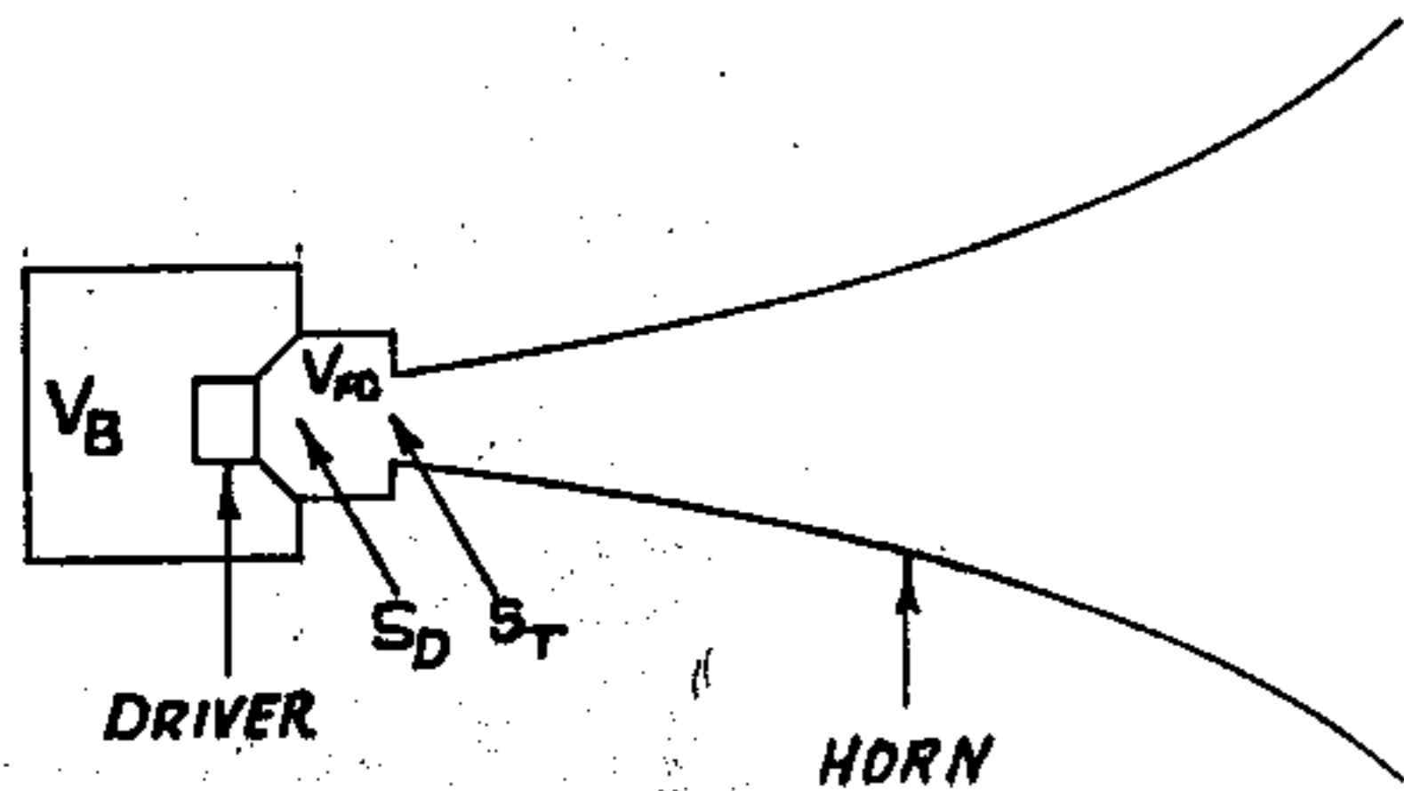
Fig. 1. Depiction of low-frequency horn-driver system. Back cavity V_B , front cavity V_F , diaphragm area S_D , and horn throat area S_T are indicated.
