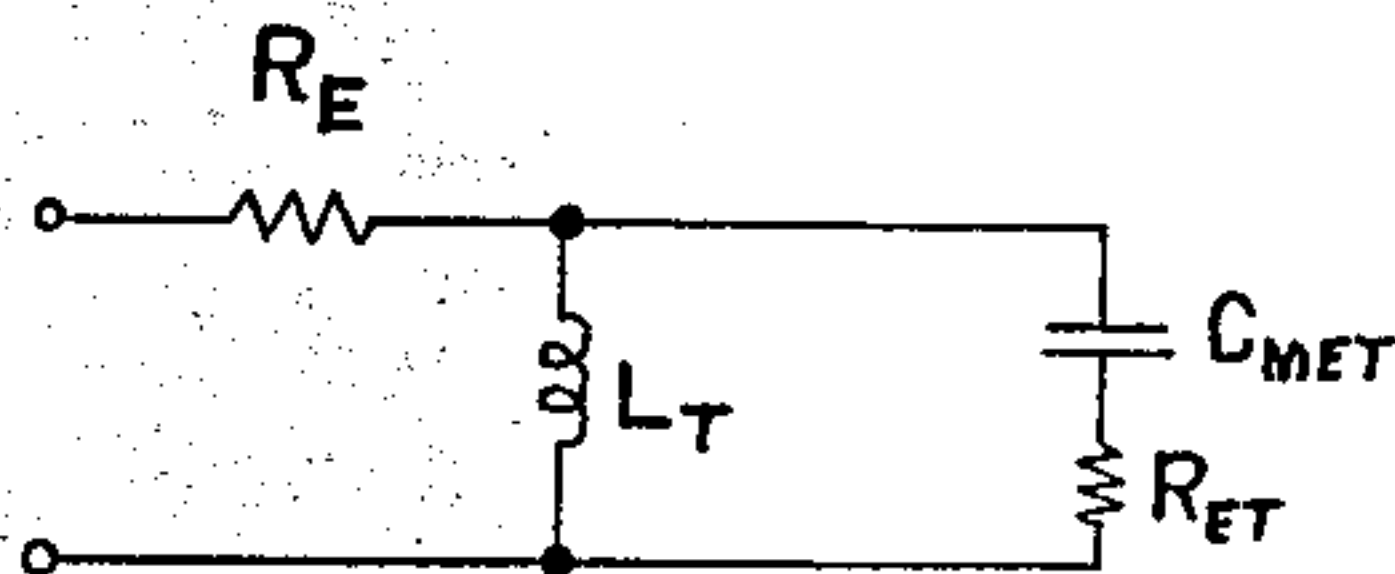
Fig. 5. Reduction of the simplified horn-driver system electrical equivalent circuit of Fig. 2. In the low frequency band but considering the effects of horn cutoff. Note that in this region both C_{MET} and R_{ET} are non-constant functions of frequency. For the case of an infinite exponential horn however, C_{MET} is constant and positive above cutoff ( f \gg f_c ). Note that L_T = L_{CEB} L_{CES} / (L_{CEB} + L_{CES}) .
