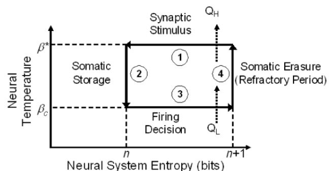
Figure 1 Carnot cycle for a pyramidal neuron having n inputs.
