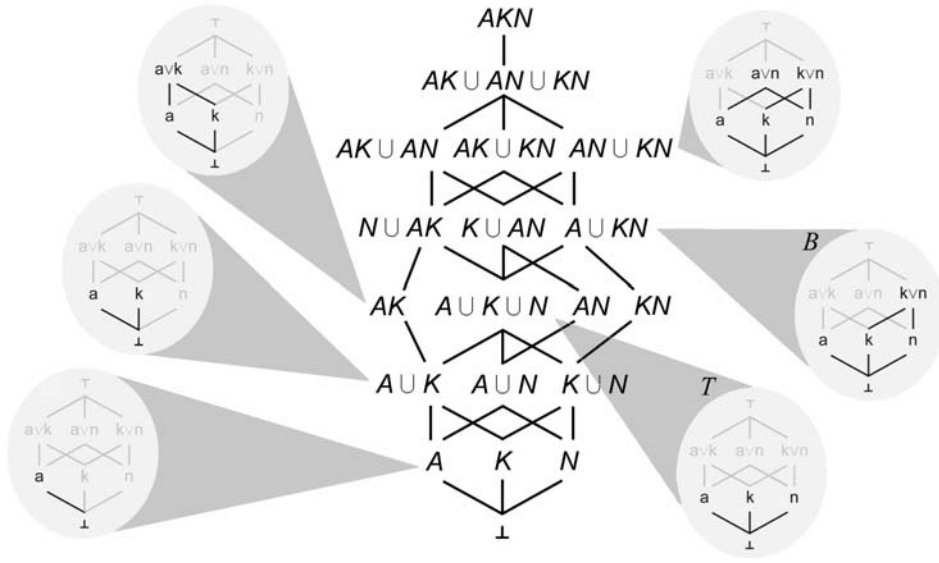
Figure 4. The lattice of all questions (center) generated by three mutually exclusive statements. Examples of the down-sets defining several questions are shown, including T and B discussed in the text (right). The ordering relation ‘is a subset of’ is applied to the down-sets of statements, so that lower questions answer higher questions.
