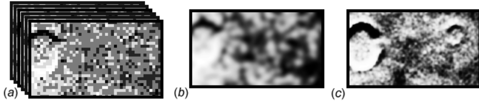
Figure 3. a. From a set of Viking Orbiter images of the Martian surface, b. the average reveals no new information, c. while the inferred high-resolution model reveals a crater not resolvable in an individual image.
