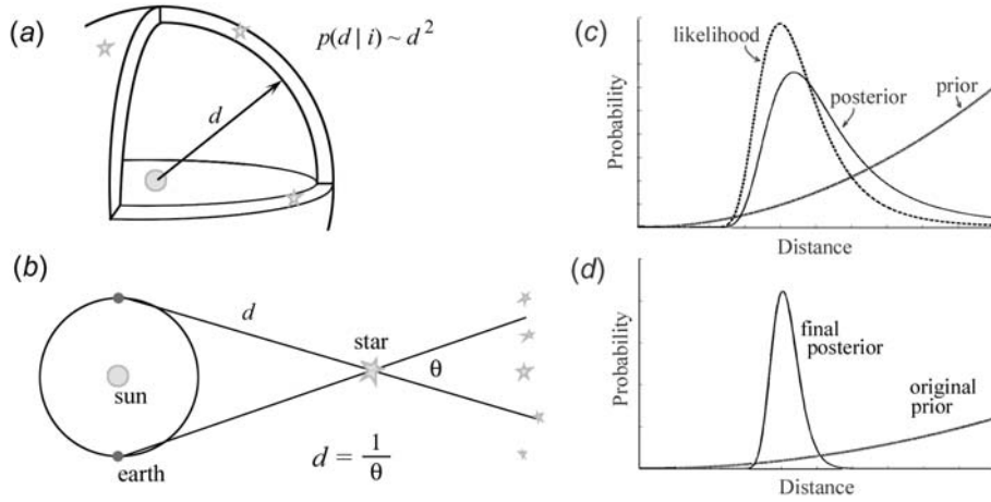
Figure 2. a. Stars uniformly distributed in space are more probable to be distant from earth than near. b. The origin of stellar parallax. c. The resulting posterior is narrower than the prior—we have learned something. d. After incorporating 5 new measurements, the posterior has grown in amplitude (compare to prior), reflecting the high probability of the solutions, and has narrowed, reflecting a more refined solution.
