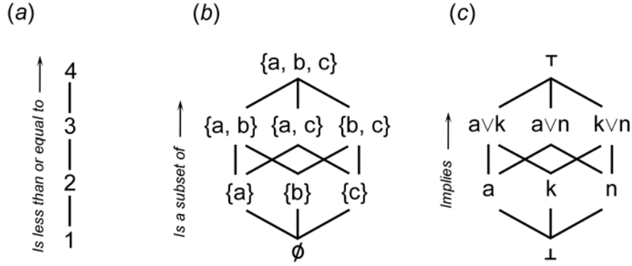
Figure 1. Diagrams of lattices described in the text. a. Natural numbers 1, 2, 3, 4 ordered by ‘less than or equal to’, b. All subsets of \{a, b, c\} ordered by ‘is a subset of’, c. Logical statements ordered by implication.
