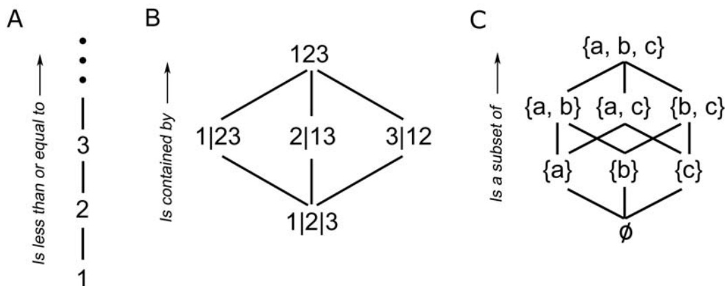
Fig. 1. Diagrams of posets described in the text. A. Natural numbers ordered by ‘less than or equal to’, B. \Pi_3 the lattice of partitions of three elements ordered by ‘is contained by’, C. 2^3 the lattice of all subsets of three elements \{a, b, c\} ordered by ‘is a subset of’.
