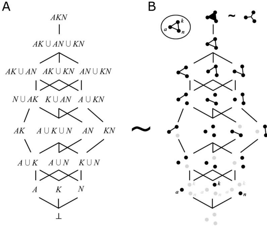
Fig. 4. The lattice of questions (A) is isomorphic to the lattice of simplicial complexes (B). The atomic questions A , K , and N are isomorphic to the three 0-simplexes. The real questions are isomorphic to the simplicial complexes that include every 0-simplex in the space. Questions are not only related to these geometric constructs, they are also isomorphic to hypergraphs. Since low-order hypergraphs look like low-order simplicial complexes, the lattice of hypergraphs with three generators is almost identical. The only exception is that instead of the 2-simplex at the top, we have the hypergraph connecting the three points (see top of B).
