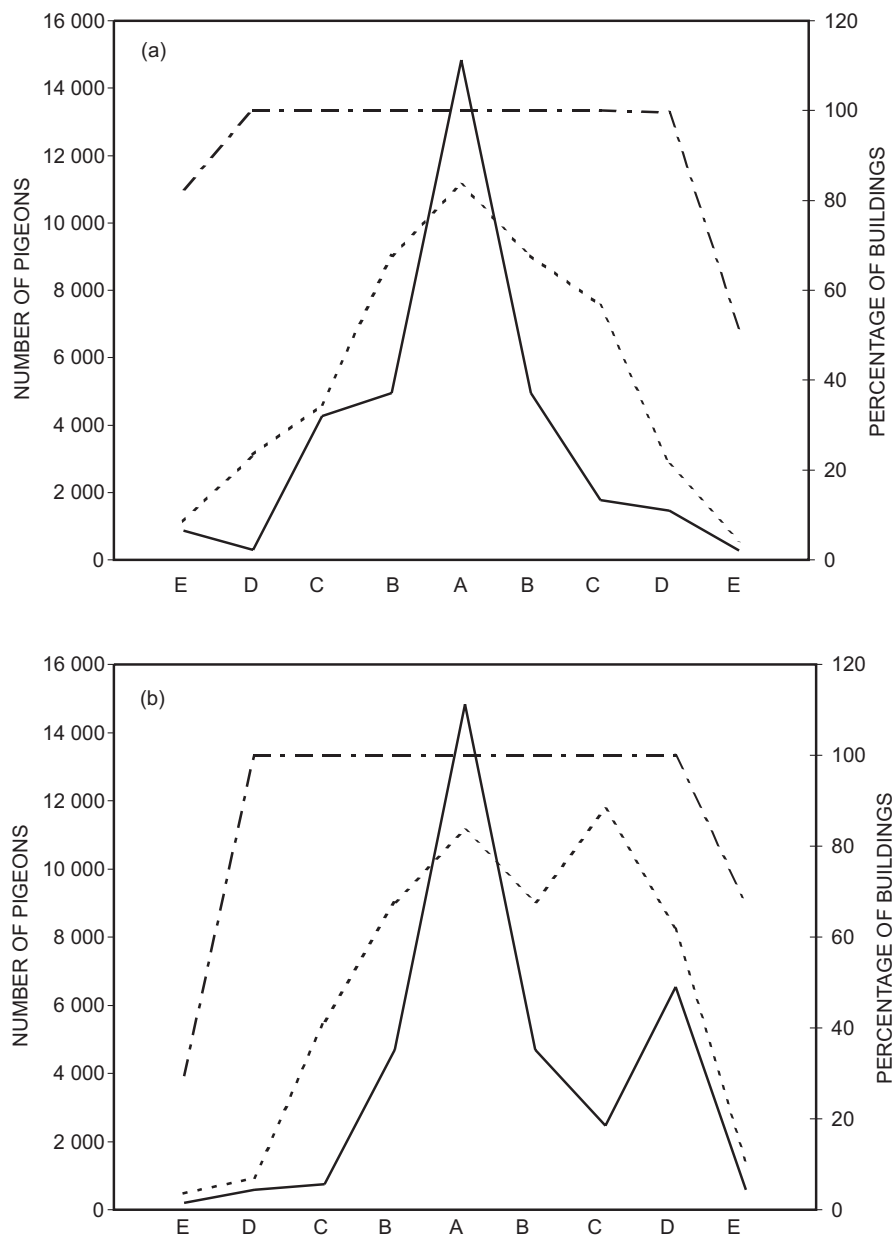
Fig. 6. Variation in pigeon numbers (solid line) along two transects across the five concentric circular areas in the centre of the city: north–south (a) and west–east (b). The dotted line shows the percentage of buildings constructed before 1936 and the broken line shows the total percentage of urban area.
