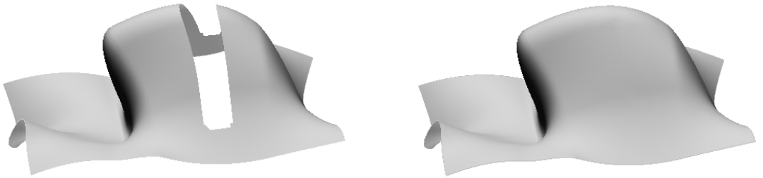
(a) A surface with a hole whose vicinity cannot be parameterized by projection (b) The non-planar hole filled using our method
