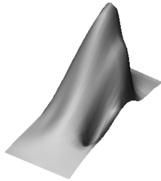
(b) The resulting surface when fitting is performed without filling the hole using singular value decomposition to obtain the least norm solution
