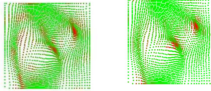
(a) Error with the blending local fits method. (b) Error with the global least squares fit method.
