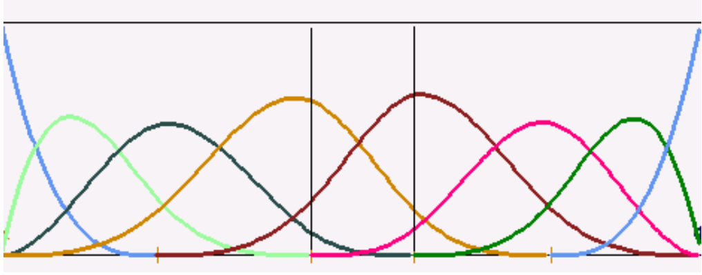
Figure 7.5. Global basis functions corresponding to the knot vector
