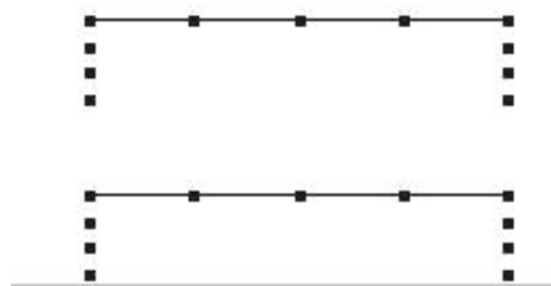
Figure 7.28. The knot vector
