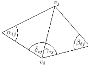
Figure 6.1. Mean-Value Coordinates
