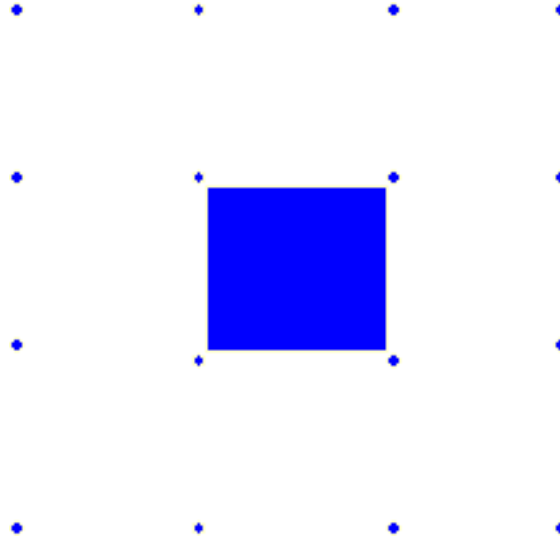
Figure 7.11. The nodes corresponding to control points of a local fit for a uniform knot vector
