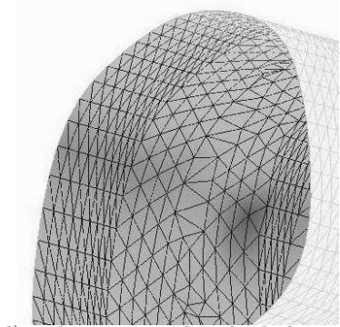
(d) The triangulated hole after completion of the hole-filling process
