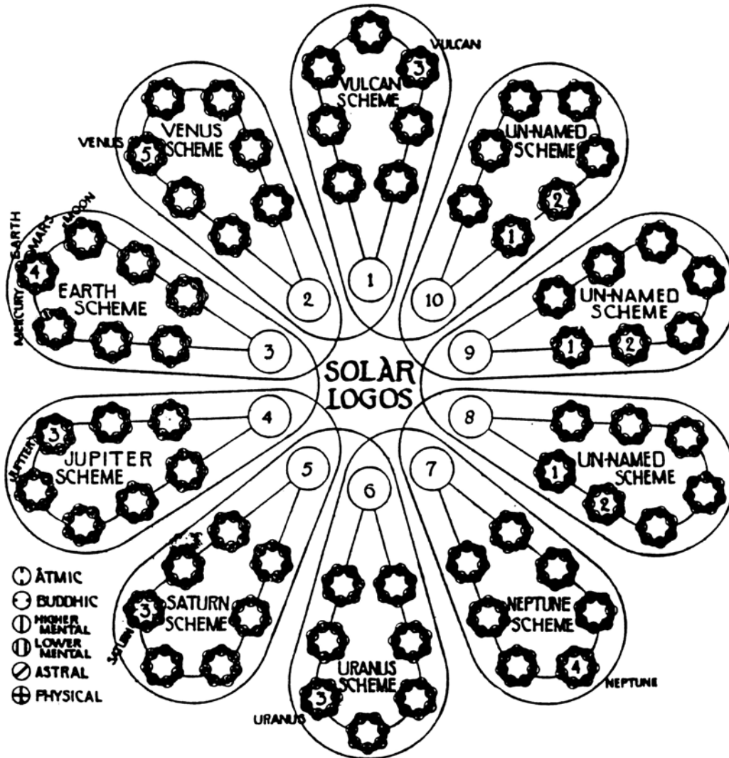
DIAGRAM VIII.—The Plan of the Solar System.
