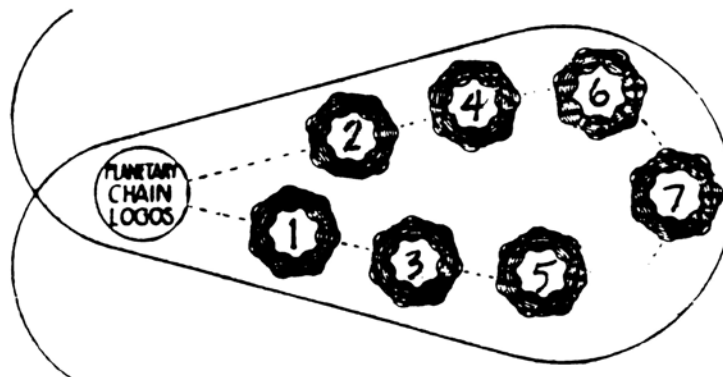
DIAGRAM VII.—The Earth Scheme of Evolution.
