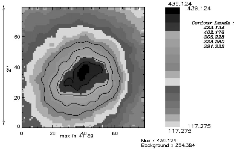
Fig. 6. Close view of the very inner coma of comet Hale-Bopp from 60 sec SK filter image of 15 January 1998. Basic data reduction, but no deconvolution processing is applied. The central brightness maximum in the coma has an oval halo and is almost resolved in its double peak seen after deconvolution.
