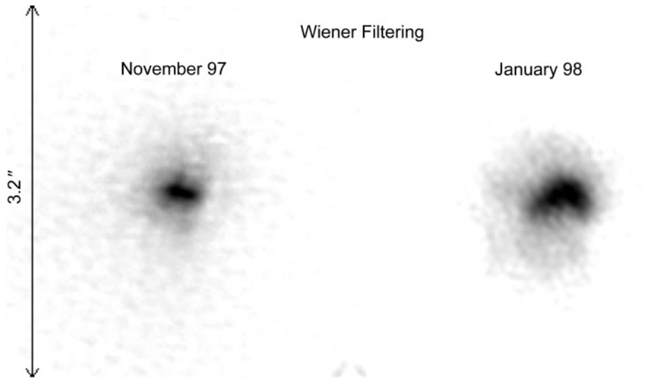
Fig. 3. Result images of the inner coma of comet Hale-Bopp using Wiener filtering with an estimated value of white noise.
