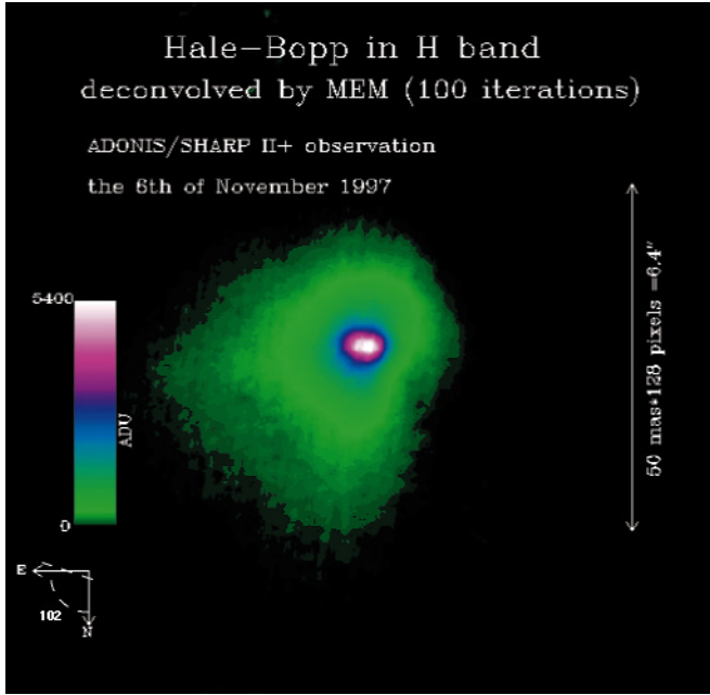
Fig. 7. Close view of the very inner coma of comet Hale-Bopp on 6 November 1997 after MEM deconvolution
