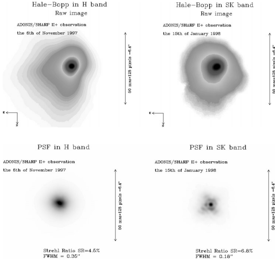
Fig. 1. Example images of comet Hale-Bopp after the basic data reduction and before deconvolution. In the H filter image of 6 November 1997 ( left ) jets are clearly visible as isophot extensions towards the east in the coma. In the SK image of 15 January 1998 ( right ) jets are less discernible. However, the near-nucleus coma shows an oval shape.
