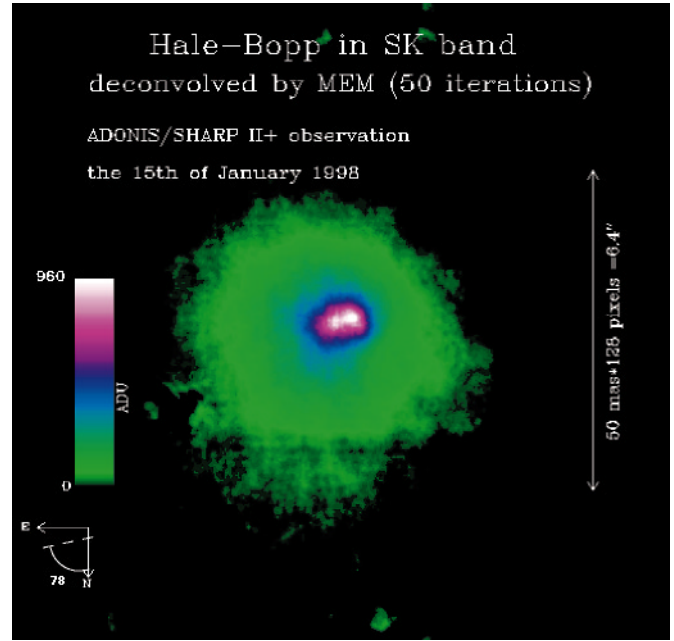
Fig. 8. Close view of the very inner coma of comet Hale-Bopp on 15 January 1998 after MEM deconvolution
