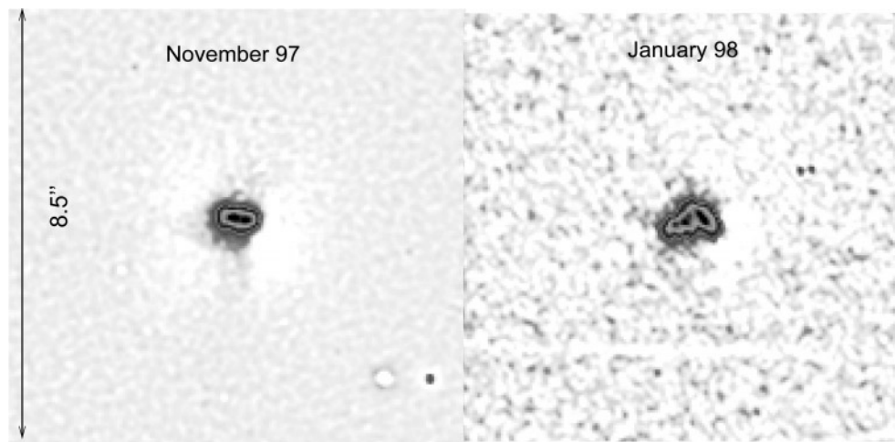
Fig. 4. Result images of the inner coma of comet Hale-Bopp using wavelet filtering
