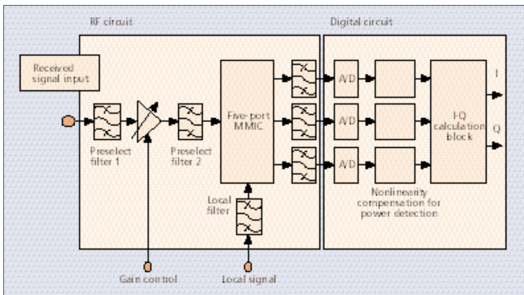
■ Figure 4. A block diagram of Sony CSL's SDR platform (SOPRANO).
