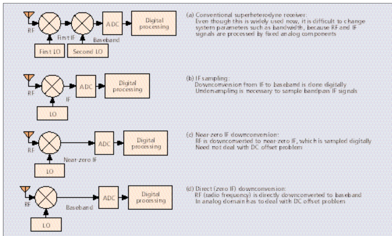
■ Figure 2. Types of down conversion in receiver.
