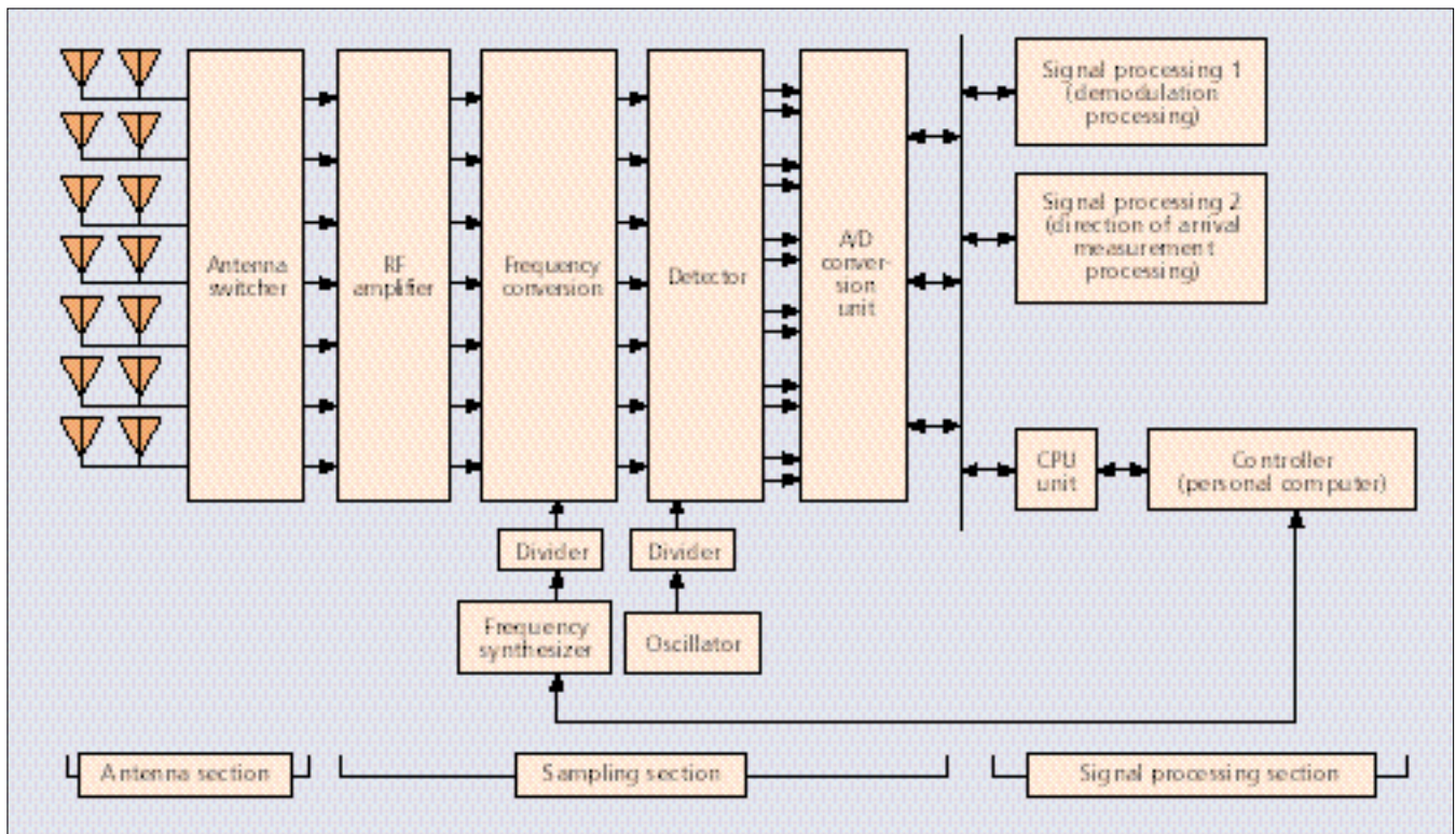
■ Figure 3. A block diagram of the prototype SDR receiver for ARIB.
