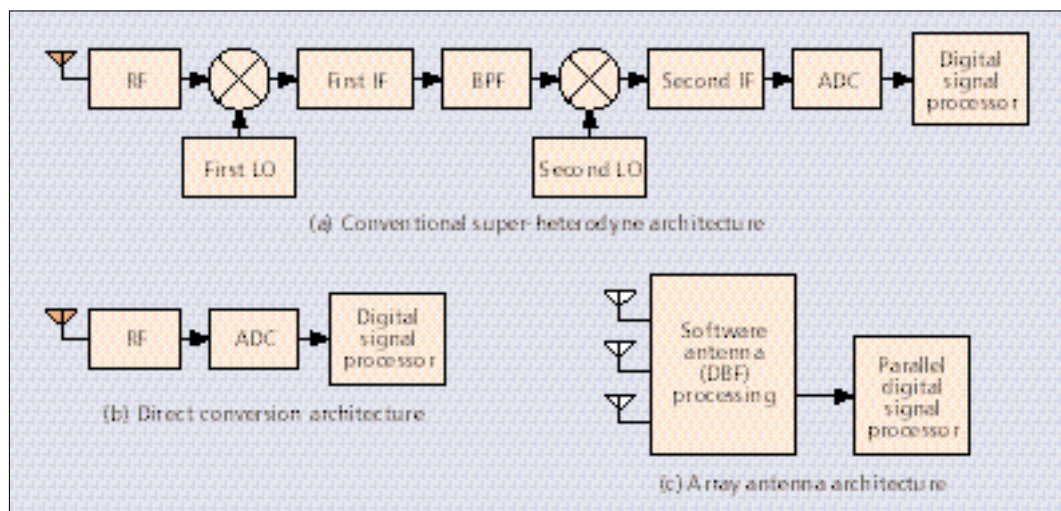
■ Figure 1. Various configurations for software-defined radio systems (receiver side).
