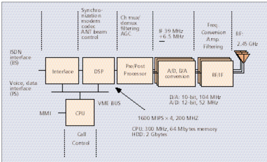
■ Figure 5. The configuration of NTT's prototype SDR station.
