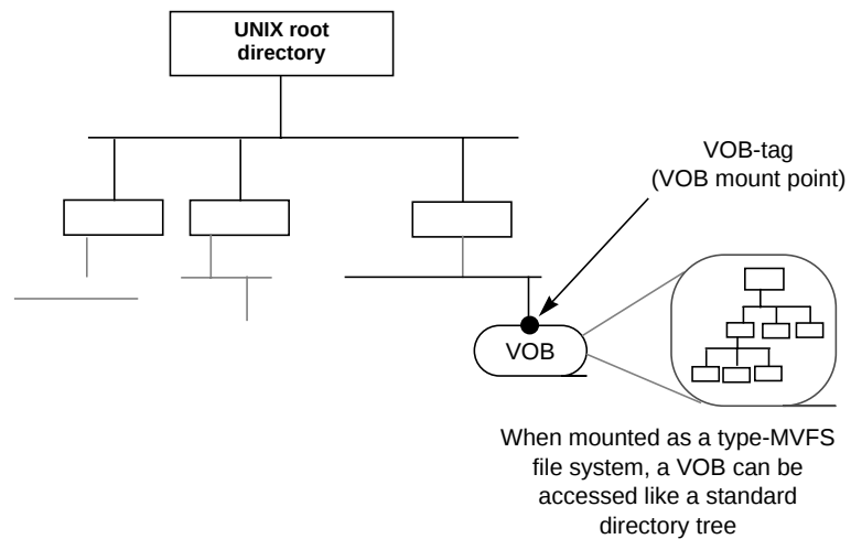
Figure 1-2 Mounted VOB
