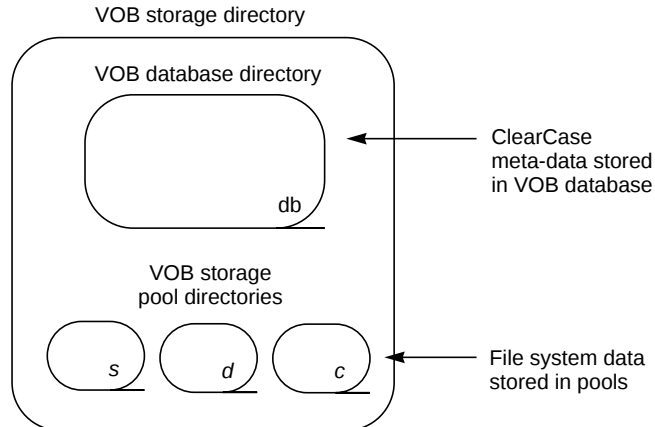
Figure 1-1 VOB Storage Directory
