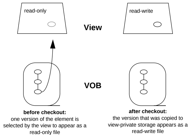
Figure 2-1 Using the checkout Command
