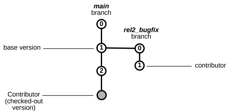
Figure 6-1 Merging Changes to a File
