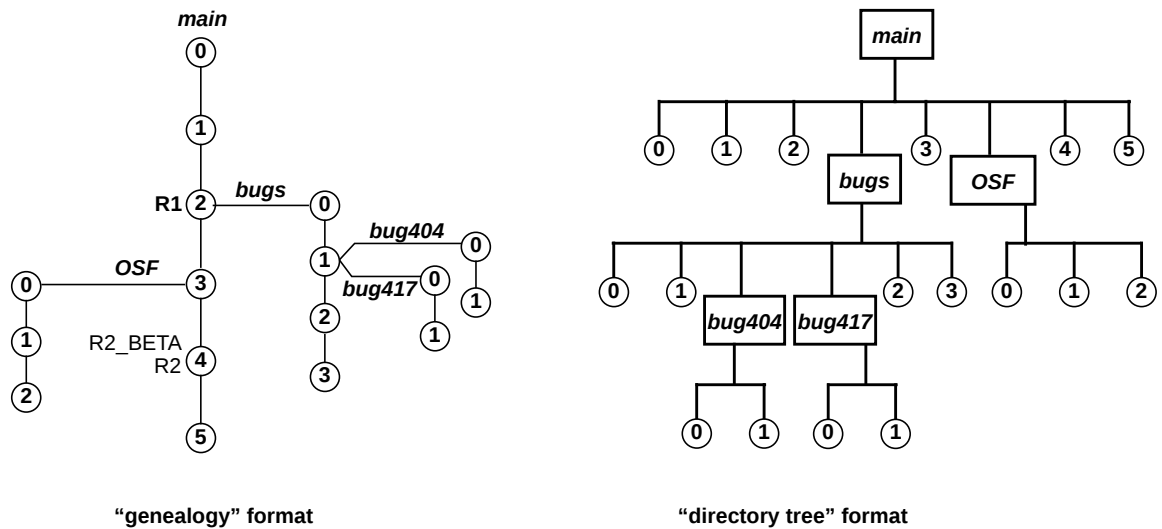
Figure 1-4 Example Version Trees
