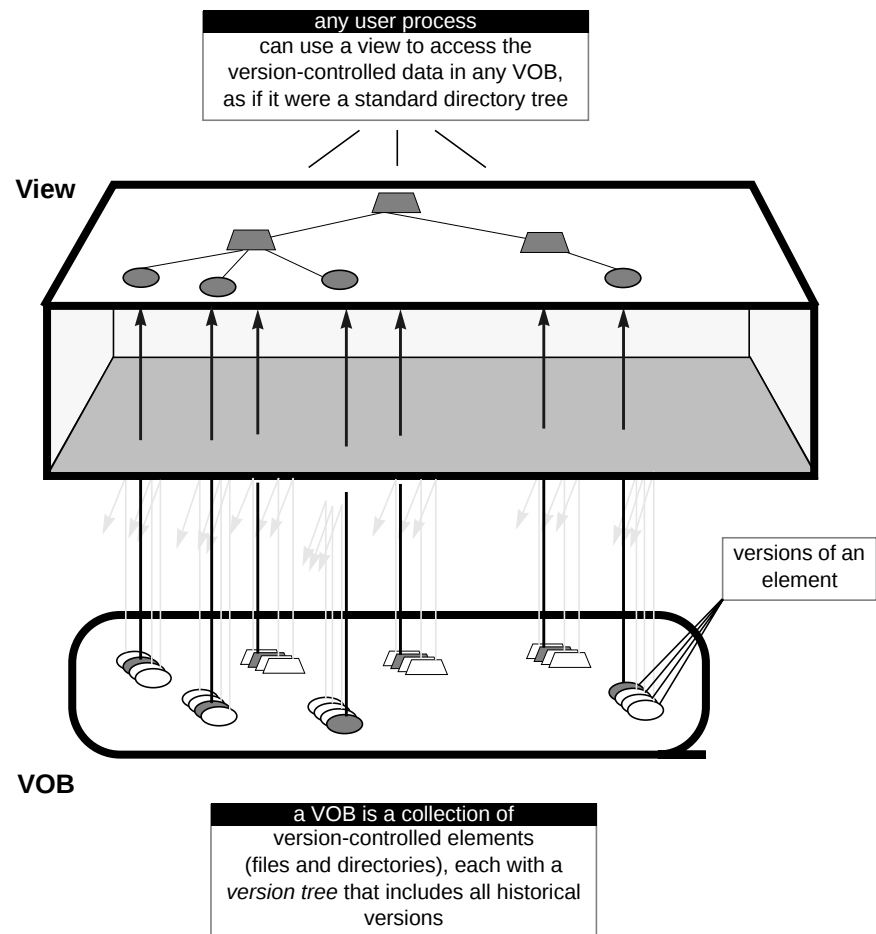
Figure 1-3 ClearCase view
