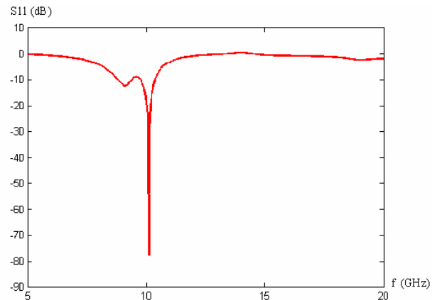
Fig. 4. The return loss of right-angle triangular slot antenna with parasitic slots.
