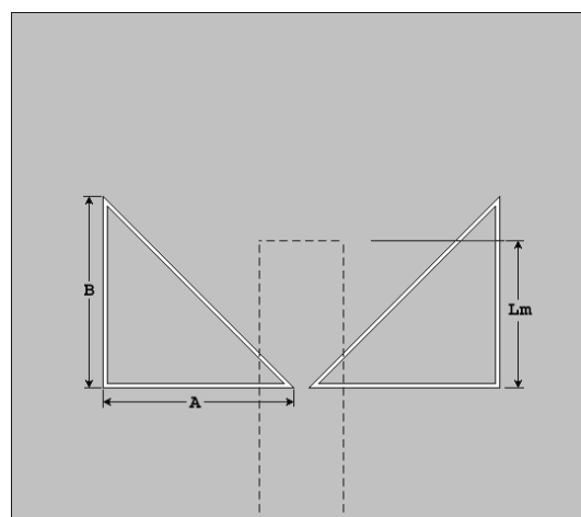
Fig. 1. The structure of Right-Angle Triangular Slot Antenna.
