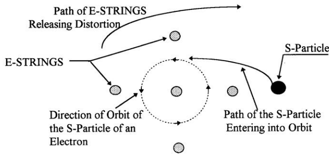
Fig. 7.2 Schematic diagram of the processes that produced an Electron from an S-Particle at the moment of the Big Bang explosion.
