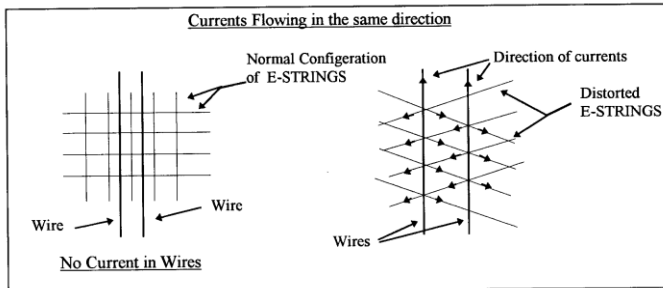
Figure 1. Currents (electrons) in the wires are flowing in the same direction, and therefore the force between the electrons is attractive. The right diagram shows that the tension created in the E-Strings by the absolute motions of the electrons is pulling the wires together.
