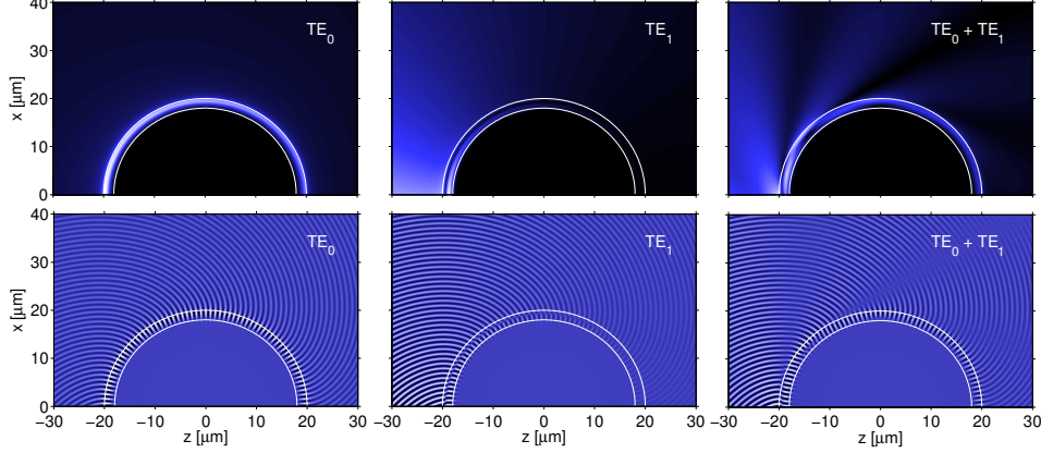
Figure 2.8: Spatial evolution and interference of the fundamental and first order TE modes, for a configuration of Table 2.3 with R = 20 \mu\text{m} . The propagation of the \text{TE}_0 mode (left), of the \text{TE}_1 mode (center), and of a superposition of these (right) is evaluated. The plots show the absolute value |E_y| (top) and snapshots of the time harmonic physical field E_y (bottom).
