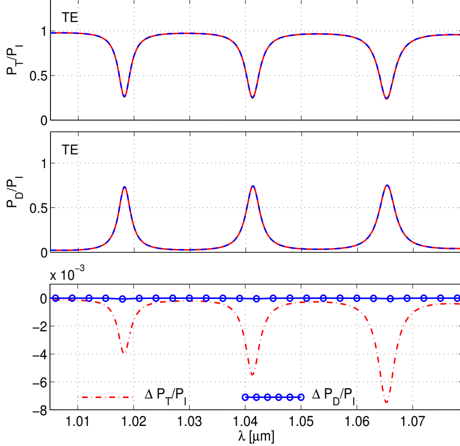
Figure 4.19: Power transmissions of the ring resonator for interchanging g and \tilde{g} . For g + \tilde{g} = 0.4 \mu\text{m} , the plots show the through power (top plot) and the dropped power (middle plot) for g = 0.25 \mu\text{m} , \tilde{g} = 0.15 \mu\text{m} (dashed lines) and g = 0.15 \mu\text{m} , \tilde{g} = 0.25 \mu\text{m} (solid lines), whereas the bottom plot shows the difference between the respective through powers (dash-dotted line), drop powers (circles) for the two settings. Note that the curves for P_D and –on the scale of the figure– also the curves for P_T are superimposed.
