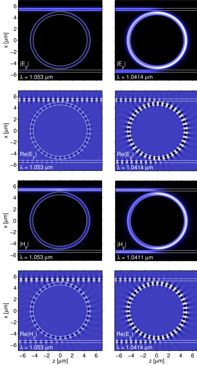
Figure 4.6: CMT results for the microring structure of Figure 4.2, local intensities (first and third row) and snapshots of the physical field (second and forth row) of the principal components of TE ( E_y ) (first and second row) and TM ( H_y ) (third and forth row) polarized waves, for an off-resonance wavelength (first column) and at a resonance (second column). For visualization purposes the coupler computational window has been extended to [z_i, z_o] = [-4, 8] \mu\text{m} .
