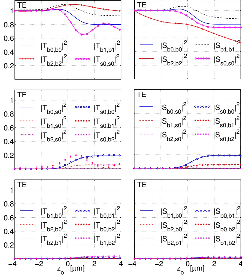
Figure 3.10: Evolution of the propagation matrix \mathbf{T} and scattering matrix \mathbf{S} for the coupler configuration with multimode bend as specified in Section 3.4.2; CMT results with four basis fields.
