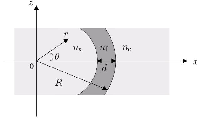
Figure 2.1: A bent slab waveguide. The core of thickness d and refractive index n_f is embedded between an interior medium (“substrate”) with refractive index n_s and an exterior medium (“cladding”) with refractive index n_c . The distance between the origin and the outer rim of the bend defines the bend radius R .
