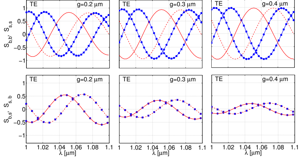
Figure 3.7: Wavelength dependence of complex valued entries of the scattering matrix S . For each separation distance, the plots in the first row show \Re(S_{b0,b0}) (line with circles), \Im(S_{b0,b0}) (line with squares), \Re(S_{s0,s0}) (solid line), \Im(S_{s0,s0}) (dashed line), and the plots in the second row show \Re(S_{b0,s0}) (circles), \Im(S_{b0,s0}) (squares), \Re(S_{s0,b0}) (solid line), \Im(S_{s0,b0}) (dashed line). \Re and \Im denote the real and imaginary parts of the complex numbers. Coupler configurations are as in Figure 3.6.
