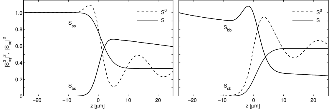
FIGURE 3. Evolution of the scattering matrix elements S_{pq}^0 and S_{pq} (absolute squares) for a coupler structure as defined in Figure 1, for a bend radius R = 30\mu\text{m} and a narrow gap of width g = 0.1\mu\text{m} . The CMT computational window is adjusted as described in Section 3, with \Delta_z = 25 , \Delta_l = 2\mu\text{m} , and \Delta_r = 20\mu\text{m} . Note that the curves display coefficients for the interaction of non-orthogonal, not necessarily normalized basis fields.
