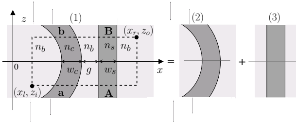
Figure 2: CMT setting for bent-straight waveguide couplers. The coupler is defined in the region [x_l, x_r] \times [z_l, z_r] . The external segments of the bent waveguide and the straight waveguide constitute the port connections. It is assumed that outside the coupler there is negligible interaction between the waveguides.
