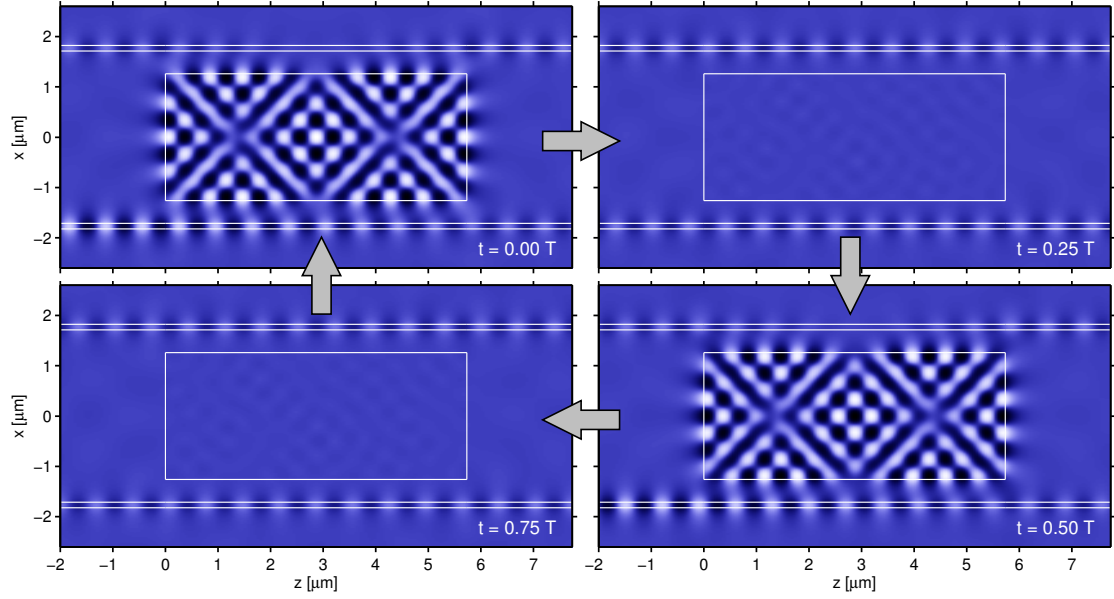
FIGURE 12. Field pattern for the pronounced resonance in Figure 11 at \lambda = 1.55 \mu\text{m} , extremal snapshots of the single electric y-component of the TE fields, at times t equally distributed over one period T . The rigorous simulation from [13] predicts relative power transmissions of P_A = 24.4\% , P_B = 25.5\% , P_C = 24.5\% , and P_D = 24.2\% .
