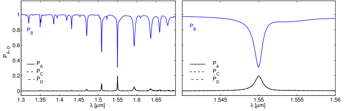
FIGURE 11. Spectral response of a resonator device according to Figure 10 with dimensions L = 5.738 \mu\text{m} , W = 2.524 \mu\text{m} , g = 0.450 \mu\text{m} , w = 0.112 \mu\text{m} for refractive indices n_b = 1.45 and n_g = 3.40 ; 2D simulations for TE polarized fields. P_A to P_D are the relative power fractions that are reflected respectively transmitted into ports A to D.
