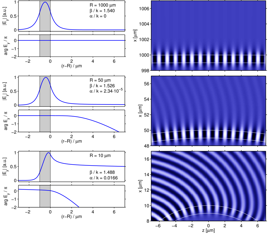
FIGURE 5. Fundamental TE modes of three bent slab waveguides with decreasing radii (top to bottom); plots of the mode profiles E_{b,y}^0 (left) and snapshots of the propagating field \mathcal{E}_y(x, z, t) at fixed time (right). Parameters are as specified in Figure 4, for \lambda = 1.55 \mu\text{m} .
