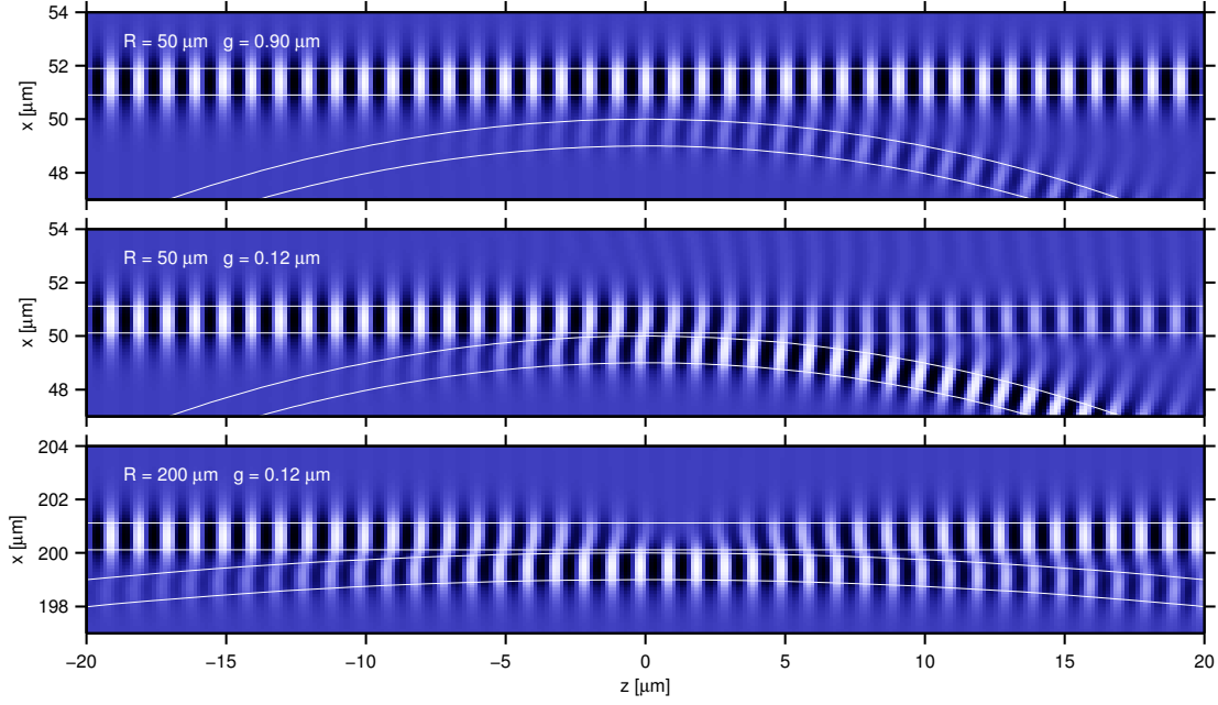
FIGURE 8. Coupled mode propagation along coupler configurations according to Figures 4, 7, for R = 50 \mu\text{m} , g = 0.90 \mu\text{m} (top), for R = 50 \mu\text{m} , g = 0.12 \mu\text{m} (center), and for R = 200 \mu\text{m} , g = 0.12 \mu\text{m} (bottom); TE polarized waves at a wavelength \lambda = 1.55 \mu\text{m} . The plots show snapshots of the physical electric field \mathcal{E}_y(x, z, t) at a fixed time, for a coupler excitation by the guided wave of the straight waveguide in the upper left port. Absolute squares of the corresponding scattering matrix entries are (|\rho|^2, |\kappa|^2, |\tau|^2) = (0.93, 0.07, 0.92) (top), (0.16, 0.83, 0.16) (center), and (0.93, 0.07, 0.93) (bottom).
