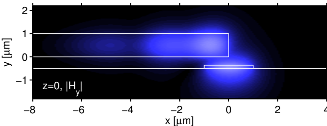
Figure 13: Vertical field cross section through the center z = 0 of the coupler structure as defined in Figure 6, for a configuration as shown in Figure 12. The gray scales correspond to the dominant magnetic component |H_y| of the TE-like polarized field; the levels are comparable with Figure 12.
