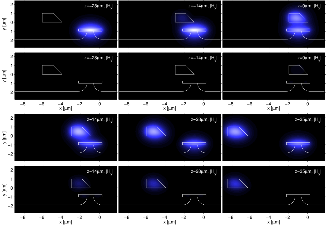
Figure 17: Transverse magnetic fields ( |H_x| , upper insets in each row, and |H_y| , below) on a series of vertical cross section planes at different z -positions for a coupler configuration according to Figure 15 with g = -2.25 \mu\text{m} . Light is launched at z_i = -35 \mu\text{m} into the mode S-TM of the straight waveguide. The gray scales of all subplots are comparable.
