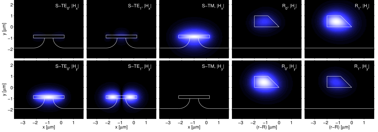
Figure 16: Vectorial mode profiles as applied for the coupled mode description of the structure of Figure 15, from left to right the three modes S\text{-TE}_0 , S\text{-TE}_1 , and S\text{-TM} of the straight waveguide, and the two hybrid ring modes R_0 and R_1 . The gray scales correspond to the absolute values of the major horizontal ( |H_x| , or |H_r| , respectively, top) and the vertical magnetic field component ( |H_y| , bottom), where the levels in each column are comparable. Cf. the remark in the caption of Figure 7 on the role of the radial polar coordinate r . Uniform parameter settings for the FMM mode analysis computations: M_s = 200 , [y_b^M, y_t^M] = [-5, 3] \mu\text{m} .
