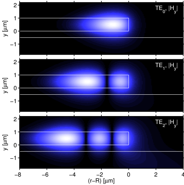
Figure 7: Profiles of the three lowest order modes supported by the disk in Figure 6(b), for a separation s = 0.5 \mu\text{m} . The plots show the absolute value |H_y| of the dominant magnetic field component for the TE-like modes. r denotes the radial coordinate in a cylindrical coordinate system with origin at the center of the disk; hence, for the vertical symmetry plane of the coupler, r - R coincides with the x -coordinate as introduced in Figures 2 and 6. Numerical parameters for the mode analysis are M_s = 200 , [y_b^M, y_t^M] = [-10 \mu\text{m} - s, 7 \mu\text{m} - s] .
