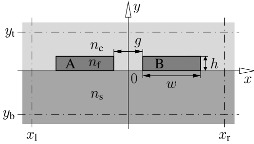
Figure 3: Two parallel straight waveguides, identical cores A, B of height h = 0.185 \mu\text{m} , width w = 3.15 \mu\text{m} , and refractive index n_f = 1.995 , on a substrate with refractive index n_s = 1.45 and covered by a material with index n_c = 1.401 . Configurations with varying gap g are considered, for TM polarized light with wavelength \lambda = 1.55 \mu\text{m} . Numerical parameters, calculation of basis modes: M_s = 120 , [y_b^M, y_t^M] = [-4, 4] \mu\text{m} ; integration of the CMT equations: \Delta x = 50 \text{ nm} , \Delta y = 37 \text{ nm} , \Delta z = 2.0 \mu\text{m} ; [x_l, x_r] = [-8, 8] \mu\text{m} , [y_b, y_t] = [-3.7, 3.7] \mu\text{m} , [z_i, z_o] = [0, L] .
