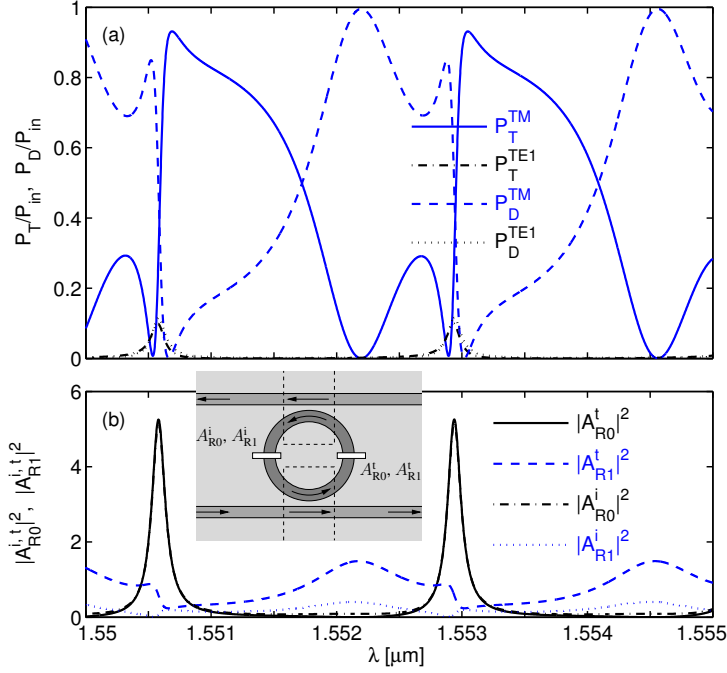
Figure 18: Spectrum of a symmetric resonator consisting of two couplers as specified in Figure 15, for an excitation by mode S-TM in one of the bus waveguides. (a): Relative power transferred to the through ( P_T ) and drop ports ( P_D ) for the two relevant polarized modes (indices TE1 and TM for S-TE 1 and S-TM) supported by the bus waveguides. (b): Squared amplitudes of the two ring modes (subscripts R0 and R1) at the input (index i) and throughput side (index t) of the cavity.
