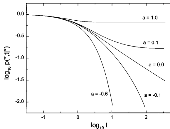
FIG. 3. The primary kinetic transition behavior in the long time asymptotic relaxation of the binding probability p(*, t|*) for several values of a with the same parameters as in Fig. 1.
