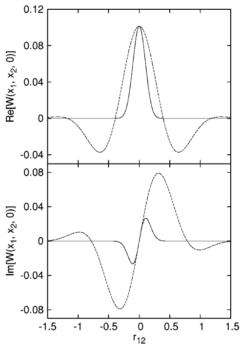
FIG. 2. Plots of the real (upper panel) and imaginary (lower) parts of W versus (dimensionless) r_{12} along the line p'_{12} = -r_{12} for \beta\hbar\omega = 0.1 (solid lines) and \beta\hbar\omega = 10 (dashed lines).
