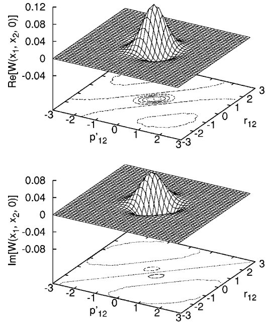
FIG. 1. Real (upper panel) and imaginary (lower) parts of W(x_1, x_2, 0) as a function of r_{12} and p'_{12} for r_c = p'_c = 1 and \beta\hbar\omega = 1 . Results are reported in terms of the dimensionless units (m\omega/\hbar)^{1/2}r and (m\omega/\hbar)^{1/2}p' .
