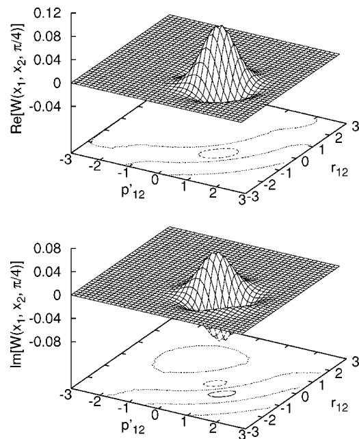
FIG. 3. Real (upper panel) and imaginary (lower panel) parts of W(x_1, x_2, t) for \omega t = \pi/4 .
