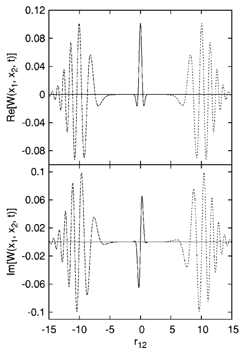
FIG. 4. Plot of W(x_1, x_2, t) function vs r_{12} for \omega t = 0 (solid line), \omega t = 7\pi/8 (long dashed line) and \omega t = 9\pi/8 (short dashed line).
