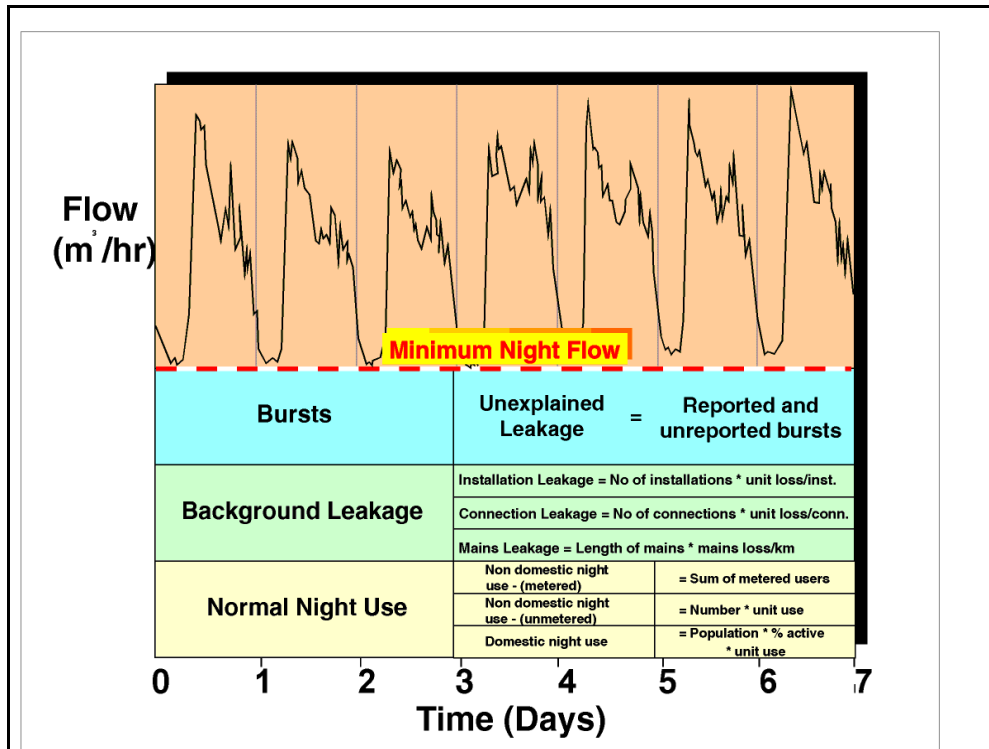
Figure 4: Components making up the minimum night-flow
