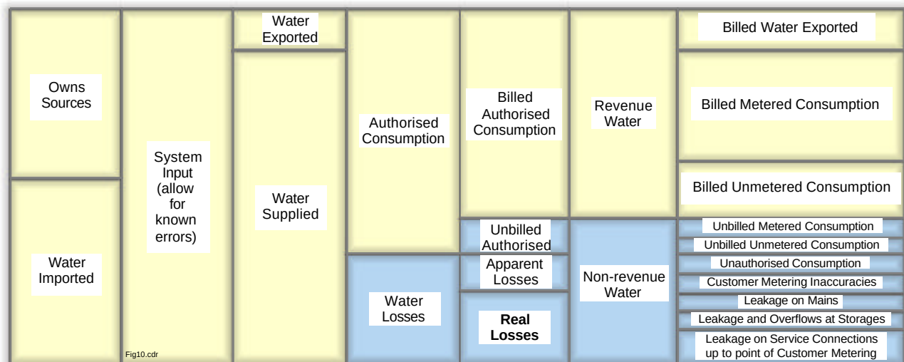
Figure 5: Main components of the water supply water balance
