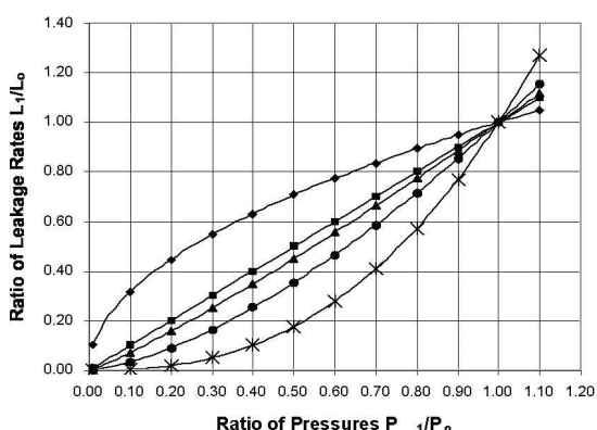
Figure 1 P_1/P_0 vs. L_1/L_0 relationships
