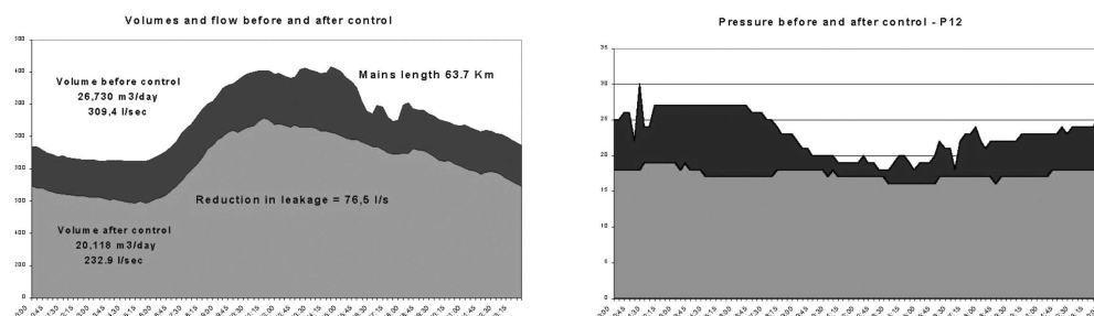
Figure 2 Reduction in leakage and unwanted demand even at low pressures
