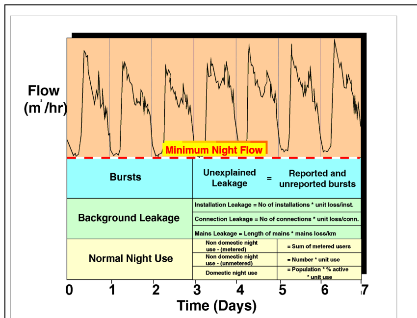
Figure 4: Components making up the minimum nightflow
