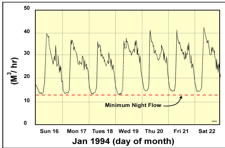
Figure 3: Example of inflow to a ZMA showing the minimum night flow
