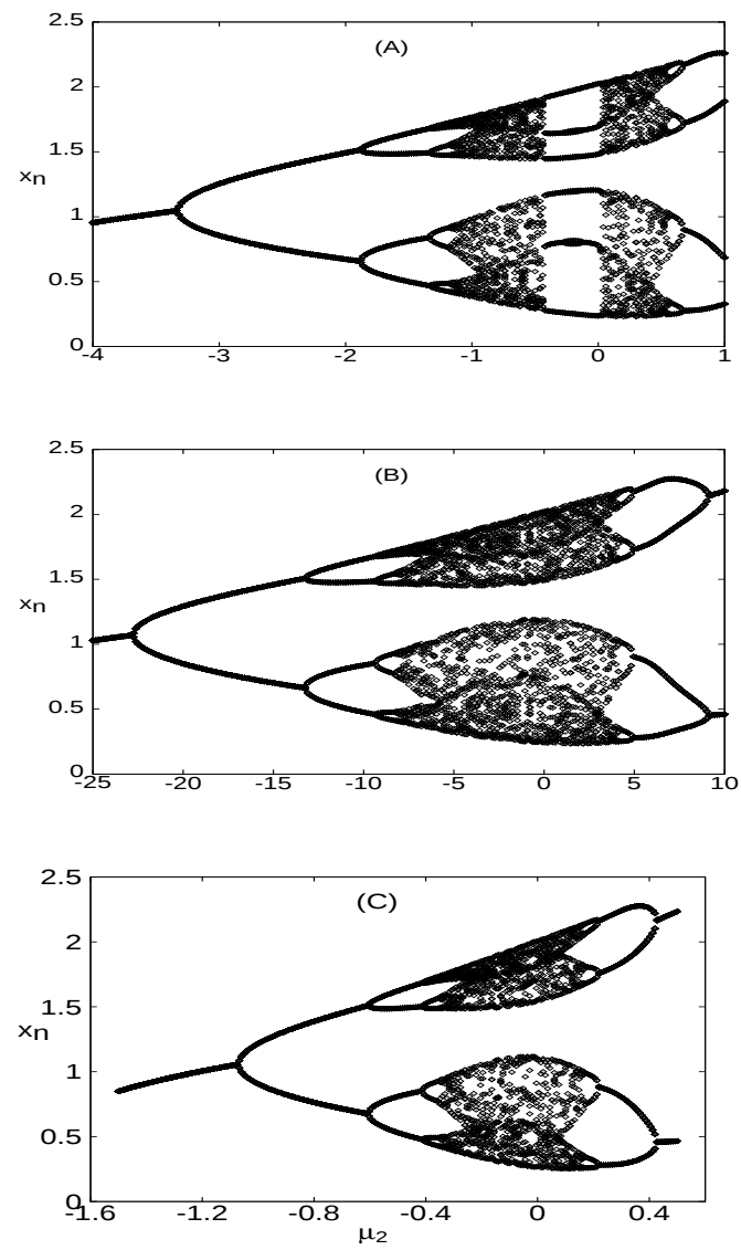
Figure 7.11: Reconstructed BD of the randomly forced sine map. (A) \kappa = 0.01 . (B) \kappa = 0.1 . (C) \kappa = 0.5 .
