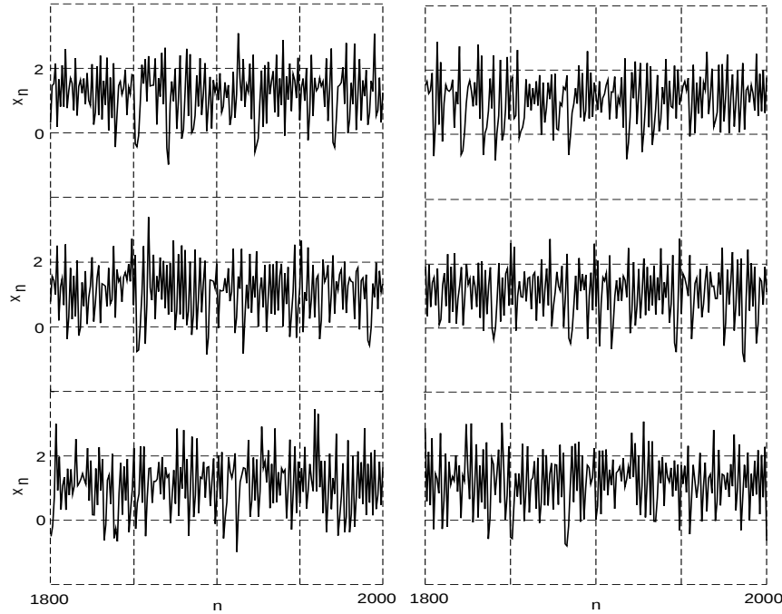
Figure 7.10: Sample time series from the sine map. Abscissas and ordinates are dimensionless.
