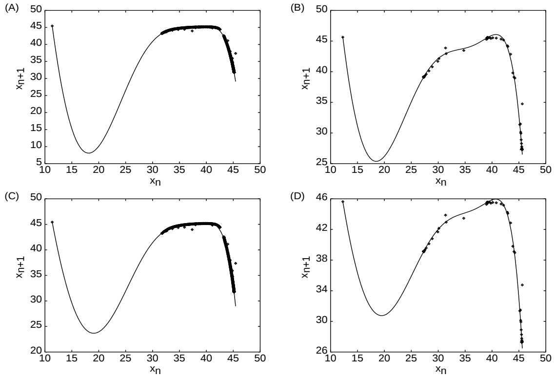
Figure 7.22: Map obtained by the identified model for the given time series. Continuous line: identified map. Discrete points: original data. (A) and (B) MODEL 1. (C) and (D) MODEL 2.
