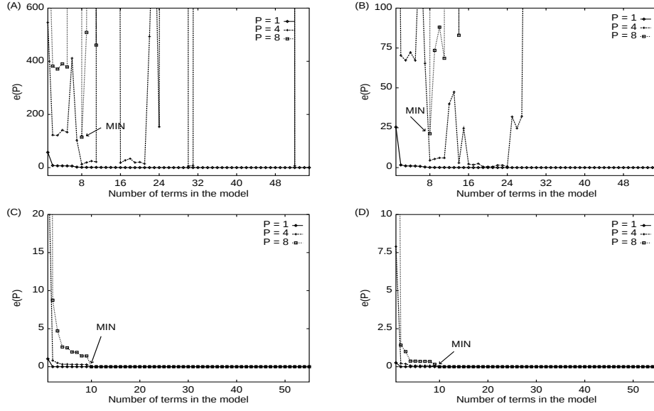
Figure 7.1: Multistep prediction error. (A) \tau = 0.8 . (B) \tau = 0.5 . (C) \tau = 0.1 . (D) \tau = 0.05 . The x-axis is the number of terms included in the model in the order given by Eq. (3.56). The minimum is indicated by the arrow.
