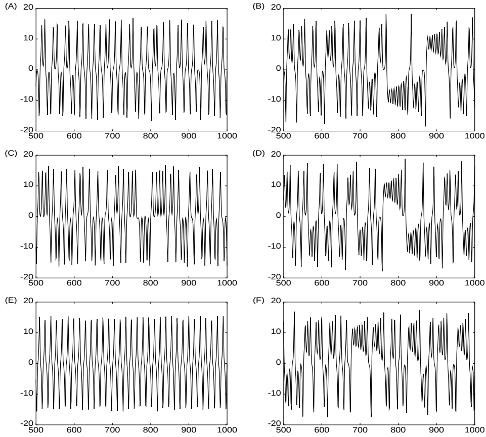
Figure 7.4: Sample time series generated by the obtained models (left side) and the corresponding time series used in estimating the parameter values of the models. (A&B) \kappa = 0.0 . (C&D) \kappa = 0.01 . (E&F) \kappa = 1.0 .
