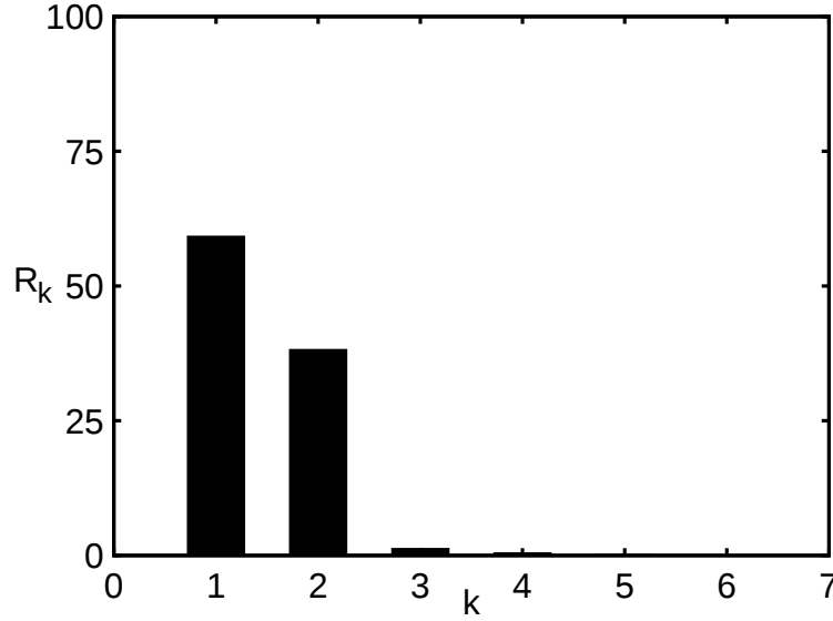
Figure 7.14: Eigenvalues (in decreasing order) expressed in relative units R_k = (\lambda_k / \sum_{i=1}^7 \lambda_i) \times 100 where \lambda_k represents an eigenvalue and k represents the order. Abscissas and ordinates are dimensionless.
