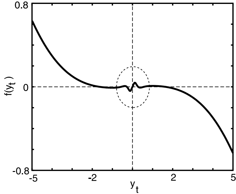
Figure 6.11: The profile of the function f(y_t) for r = 2 .
