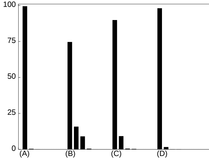
Figure 7.12: Eigenvalues. (A) \kappa = 0 . (B) \kappa = 0.5 and N = 1000 . (C) \kappa = 0.5 and N = 10000 . (D) \kappa = 0.5 and N = 20000 .
