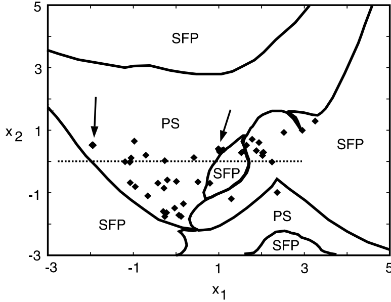
Figure 6.4: The local bifurcation structure of \tilde{g}(\cdot; \mathbf{w}) relative to the first two eigenvectors of the sample covariance matrix. The x_1 - axis is spanned by the first eigenvector while the x_2 - axis is spanned by the second eigenvector. PS denotes region of (pseudo -) periodic solutions and SFP denotes region of stable fixed point solutions. The scattered points are the projections of the time series onto this principal plane.
