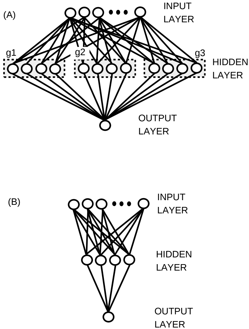
Figure 5.1: (A) The composite network made up of the three predictor functions \tilde{g}_1 , \tilde{g}_2 , and \tilde{g}_3 . The inner weights are unchanged while the outer weights are given by Eq. (5.11). (B) When the inner weights of the three networks are the same, the composite network can be trimmed to make the number of hidden units equal to that of the predictor functions. For this case, the outer weights are given by Eq. (5.12).
