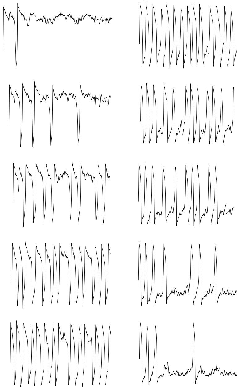
Figure 7.17: Sample time series. First 1000 data points of the time series used in reconstructing the BD of the FHN system. The presence of noise causes spiking events even for parameter values corresponding to the excitable region of the model.
