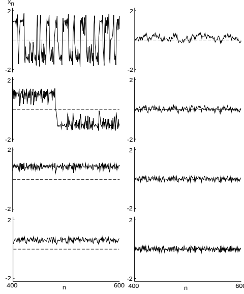
Figure 3.17: Time series for \kappa = 0.2 . Data points from the 400th to 600th iteration of S_2 to S_9 (from top to bottom, left to right).
