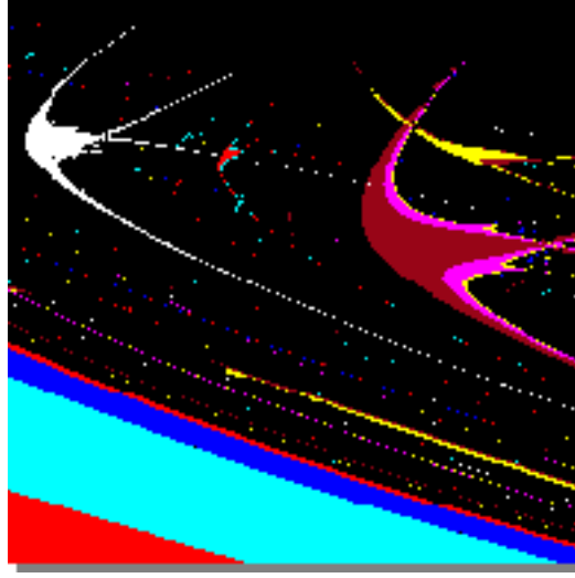
Figure 5.3: Reconstructed bifurcation diagram of the Hénon map on the linear subspace defined by Eq. (5.11) in the parameter region p_1 \in [1.15, 1.548] and p_2 \in [0.0, 0.398] . See Table 5.1 for the color coding.
