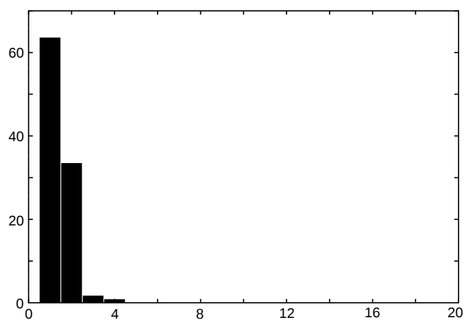
Figure 7.18: Eigenvalues of the covariance matrix form from the estimated parameter values in relative values |\text{eigenvalue}| / \sum \text{eigenvalue} \times 100 \% .
