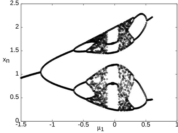
Figure 7.9: Reconstructed BD of the unforced sine map.
