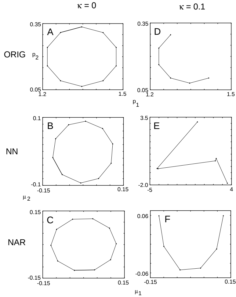
Figure 8.1: Parameter sets used in generating the time series (A & D). Projections of the estimated model parameter values onto the two principal eigenvectors for NN-based (B & E) and NAR-based (C & F).
