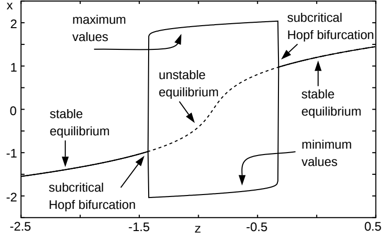
Figure 7.16: Bifurcation diagram of the FitzHugh-Nagumo equation. The other parameters are fixed: a = 0.7 , b = 0.8 , and c = 3.0 .
