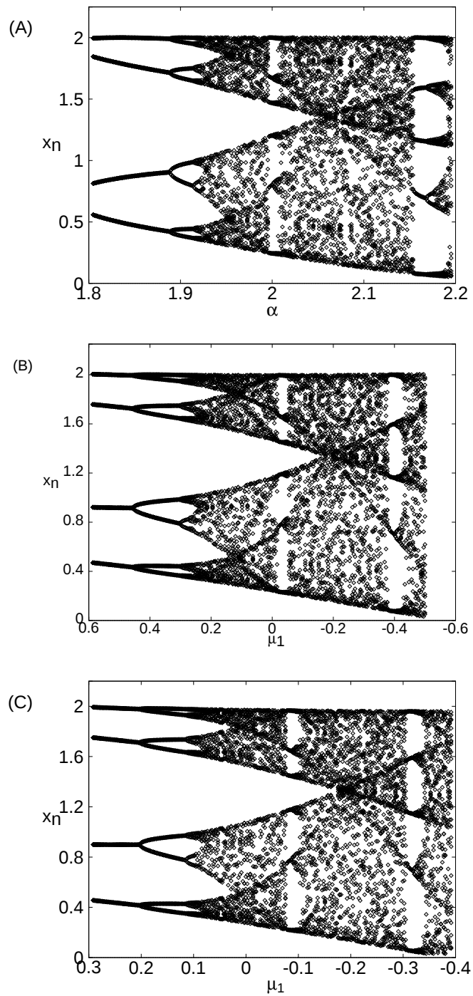
Figure 7.13: Bifurcation diagram of the sine map with respect to \alpha . (A) Original BD. (B) Reconstructed with \kappa = 0 . (C) Reconstructed with \kappa = 0.5 .
