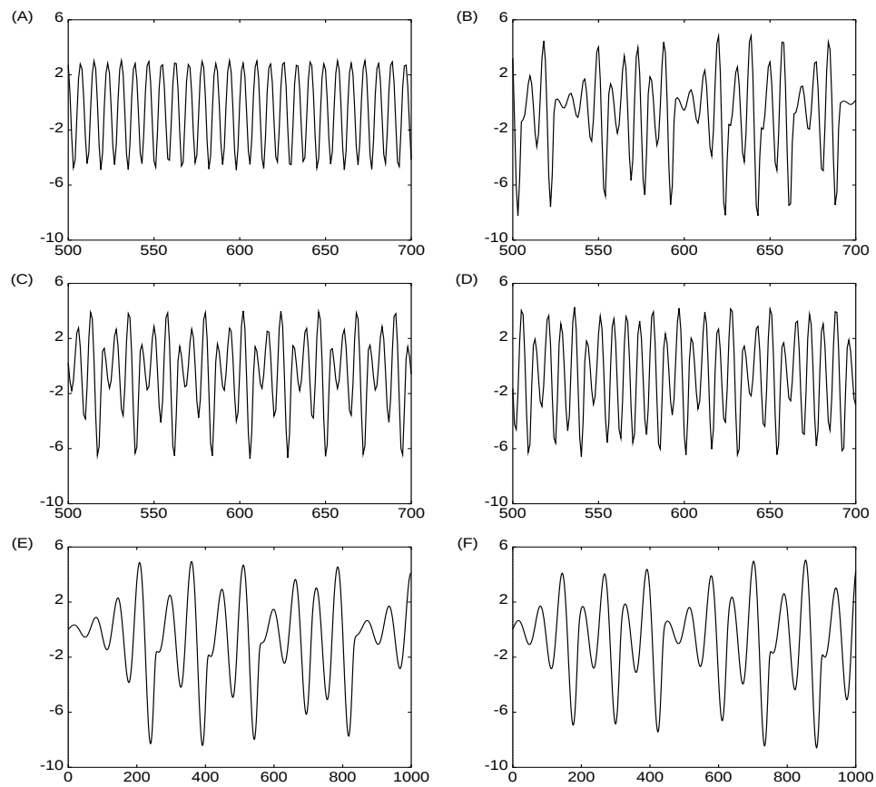
Figure 7.2: Sample time series generated by the obtained models (left side) and the corresponding time series used in estimating the parameter values of the models. (A)-(D) \tau = 0.8 . (E) and (F) \tau = 0.1 .
