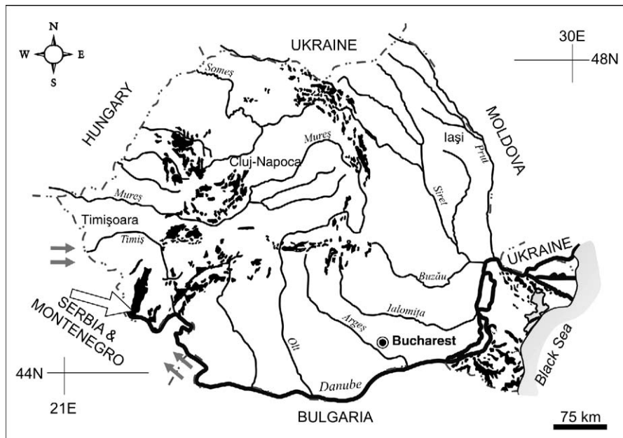
Fig. 1. The map of karst rocks (solid black shading) outcropping in Romania and location of Poleva cave (indicated by the large white arrow). The small grey arrows show the directions of the main directions of atmospheric circulation.
