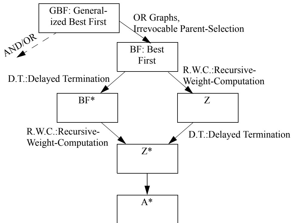
Figure 3: Pearl's Hierarchical Diagram.
