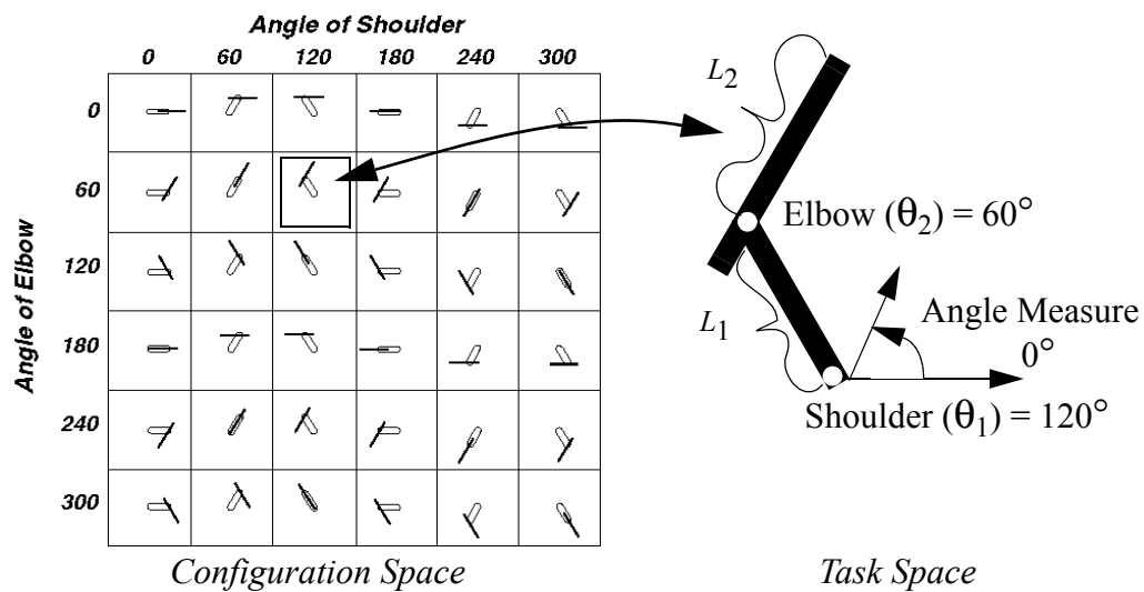
Figure 18: One Configuration.
