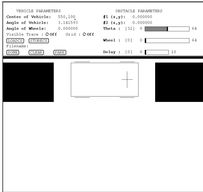
Figure 38: Simulation Interface.
