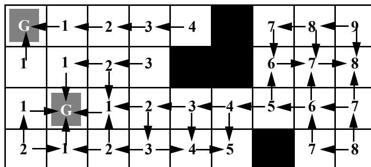
Figure 84: Paths for Two Actors - Two Scenarios Each.
