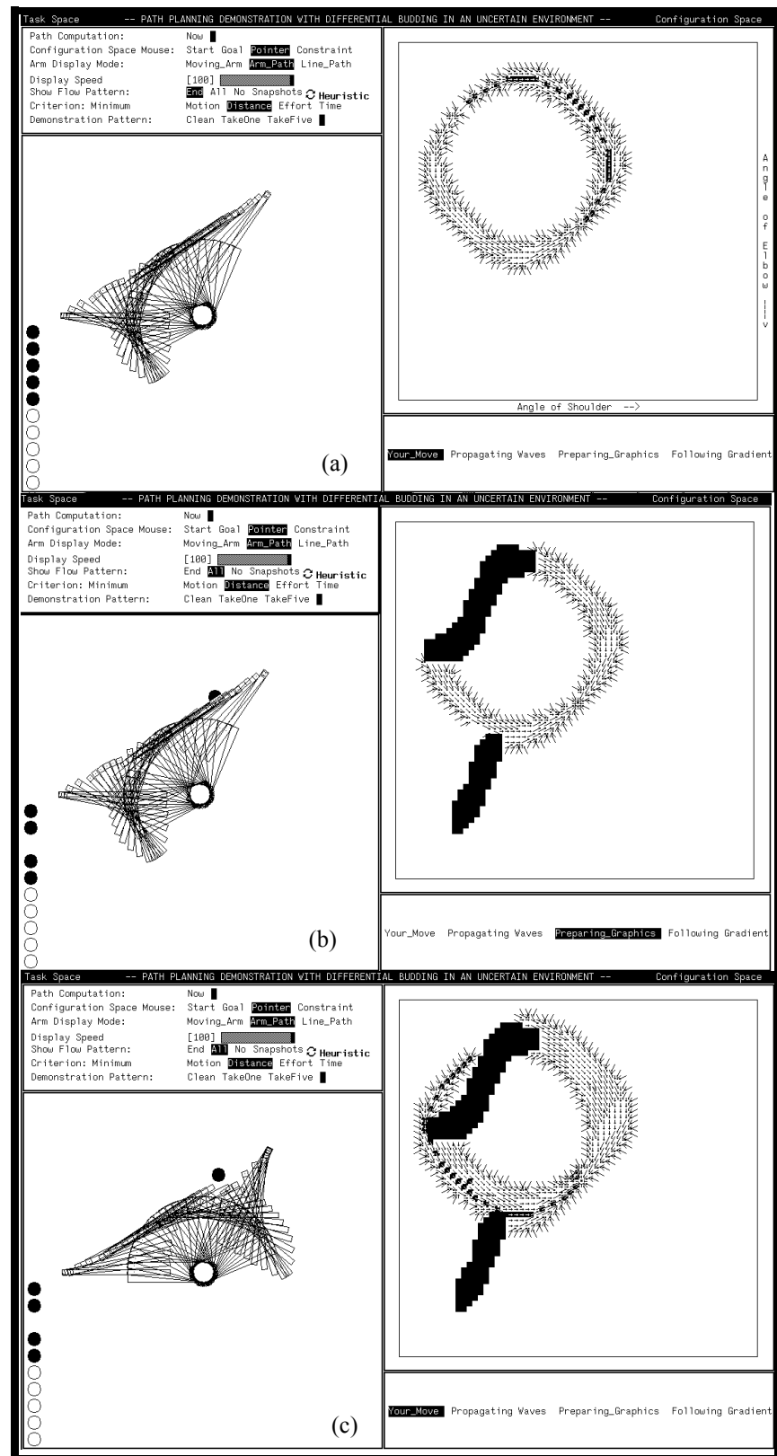
Figure 77: Admissible Heuristic Guides Search and Adapts to a New Obstacle.
