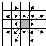
Figure 23: 16-Connected Neighborhood.
