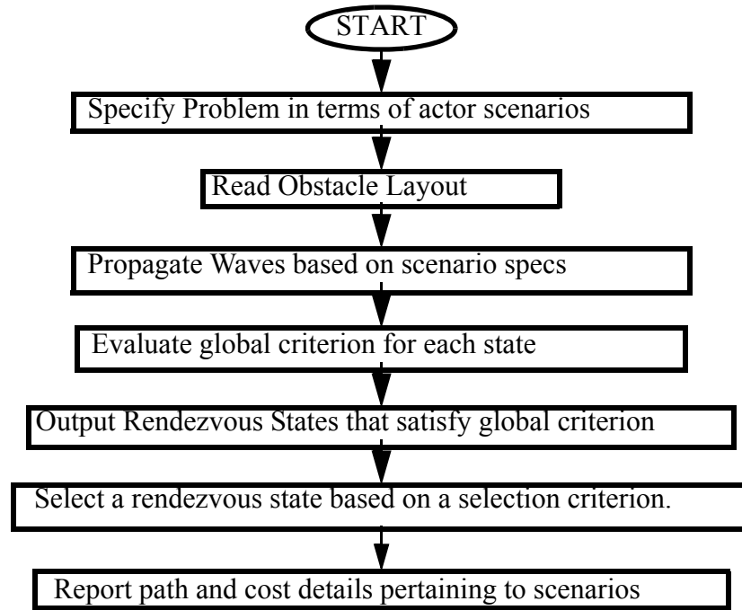
Figure 81: Rendezvous Planning.
