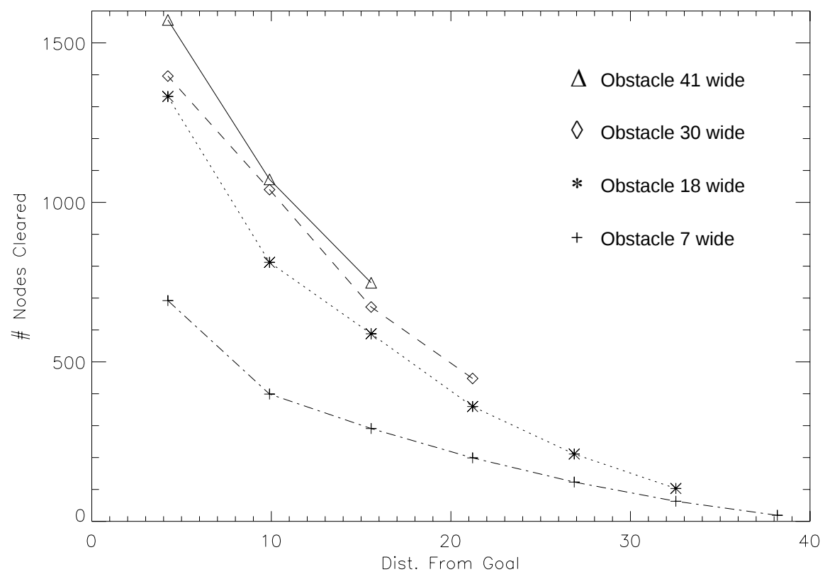
Figure 80: Obstacle Effects.
