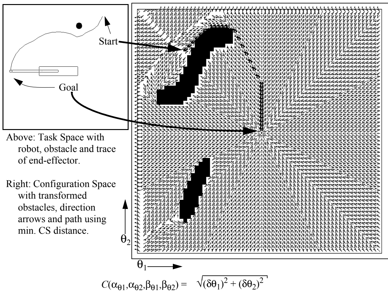
Figure 25: Least Communication.
