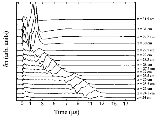
FIG. 10. Temporal evolution of the ion waves excited by suprathermal ion bunch taken at different underdense z positions at r \approx 5 cm. In the measurements the incident microwave is irradiated with a pulse width 85 ns.
