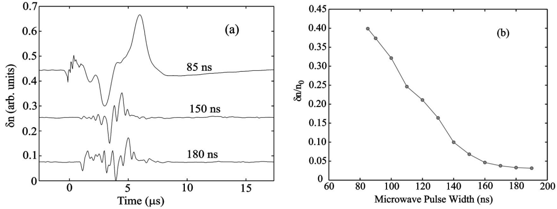
FIG. 6. (a) Temporal evolution of density perturbations ( \delta n ) with incident microwave pulse width of 85 ns, 150 ns, and 180 ns. (b) Amplitude variation of density perturbations ( \delta n/n_0 \equiv peak to peak value) as a function of the incident microwave pulse width.
