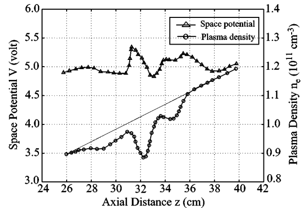
FIG. 8. Density cavity observed at resonant region (bottom trace), corresponding positive space-potential (top trace), and schematic line of density (middle trace) in the absence of microwave pulse.
