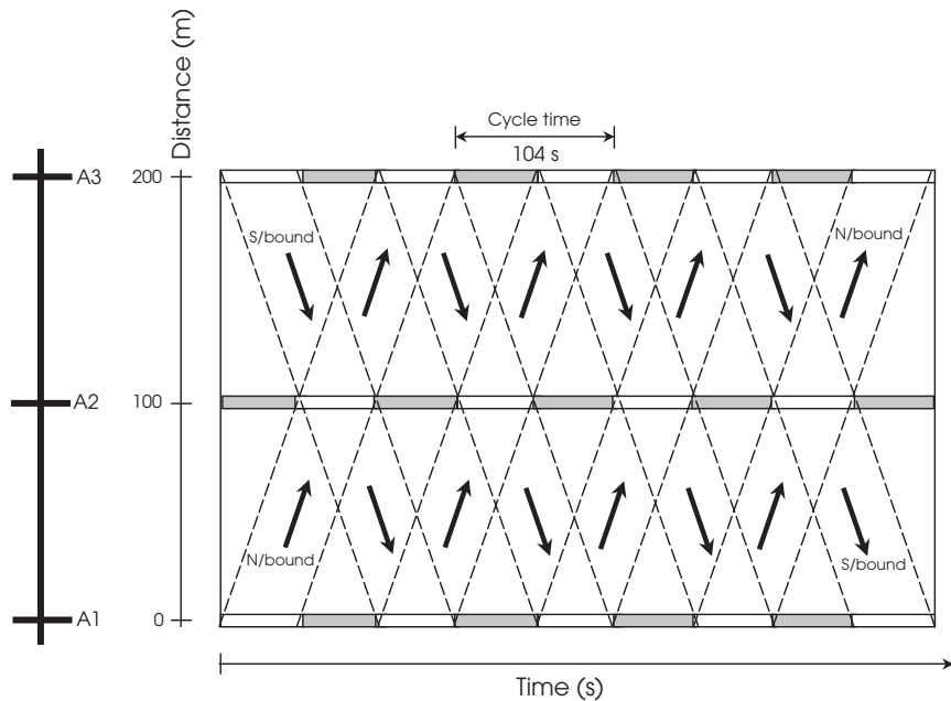
Figure 5.34 Illustration of time-distance diagram for Example 5.7.
