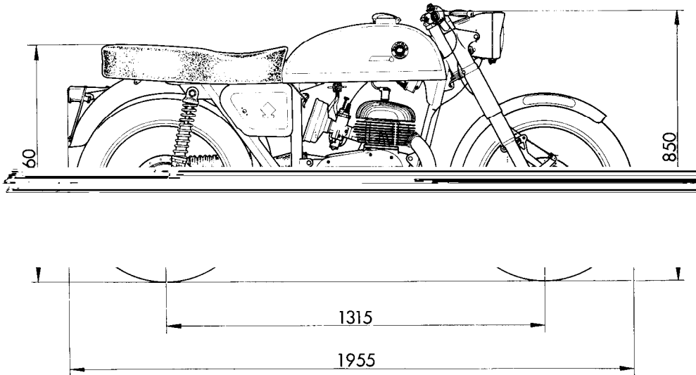
Fig. 36. — Overall dimensions.
