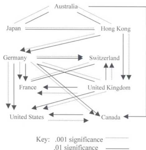
A: Pattern from TETRAD II
