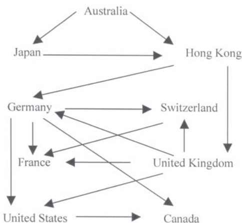
B: DAG from SL^* and TETRAD II
