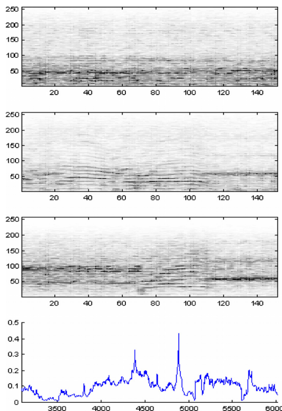
Figure 3 Graphical evidence relating to the “Play” utterance (see text). For the spectrograms, the x axis denotes frame number; at 8820 samples/sec, each frame is 512 samples long and is stepped (advanced) 64 samples from the previous one; so each x unit corresponds to a time interval of one frame step, namely 64/8820 = 0.007256 s. The y axis denotes the frequency band; each y unit corresponds to a frequency interval of 4410/256 = 17.23 Hz. Top to bottom [(a)–(d)]: (a) Spectrogram of Track 7 from t_{7pm} = 15 : 52.27 to 15:53.43 . Note the region 0 < x < 70 . (b) Spectrogram of Track 7 from t_{7pm} = 15 : 55.87 to 15:57.03 , precisely 3.60 s after part (a). Note the region 70 < x < 150 . (c) Spectrogram of Track 2 from t_{2pm} = 4 : 59.22 to 5:00.29 , showing the elision of one disk groove (3.60 s) of t_{7pm} , so that “Get the trucks out of the way.” becomes “. . . ay.” The scale of this figure has been stretched by a factor 1.08 to match the local speed ratio between Track 2 and Track 7. (d) Pattern cross correlation of Track 2 from t_{2pm} = 4 : 59.22 to 5:00.46 (of which the first 1.07 s is shown in (c)) against Track 7 from t_{7pm} = 15 : 42.80 to 16:05.25 . The peak at x = 4404 is due to the 0 < x < 70 region of part (c); that at x = 4900 is due to the x > 70 region. The separation between the peaks is 3.599 s. (The x value denotes PCC time shift measured in frame steps of 0.007256 s each.)
