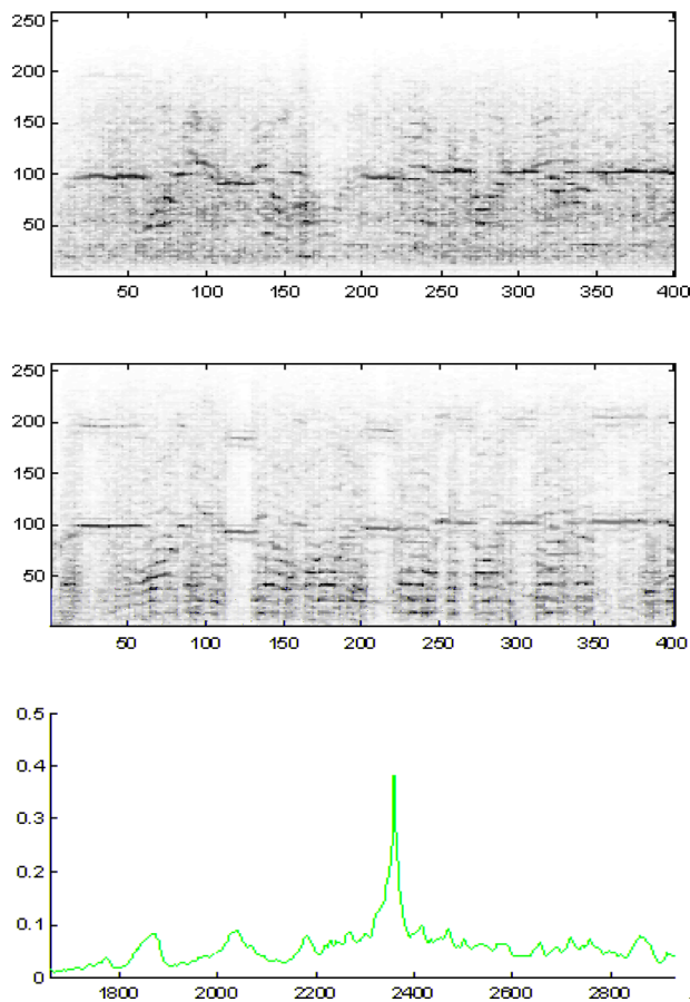
Figure 7 Spectrograms and pattern cross-correlation (PCC) plots for putative crosstalk “YOU.” Axes and units are as defined in Figure 3. From top to bottom [(a)–(c)]: (a) Spectrogram of Track 1 from t_{1pm} = 6 : 49.36 to 6:51.96 , stretched by a factor 1.012 for best local speed match to Track 7. (b) Spectrogram of Track 7 from t_{7pm} = 16 : 51.08 to 16:53.68 . (c) PCC of “YOU” utterance, for Track 1 ( t_{1pm} = 6 : 49.36 to 6:51.96 ) against Track 7 ( t_{7pm} = 16 : 44.98 to 16:57.08 ), plotted for best local stretch of Track 1 by a factor 1.012. The peak at x = 2360 is located at t_{7pm} = 16 : 51.08 .
