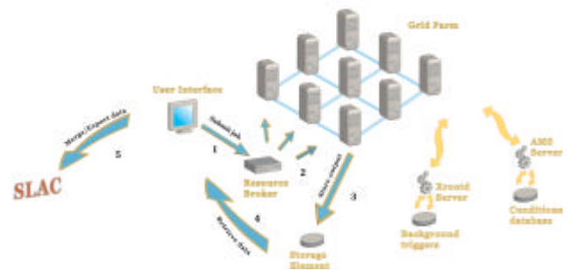
Fig. 2: BaBar simulation production model implemented in Italy
