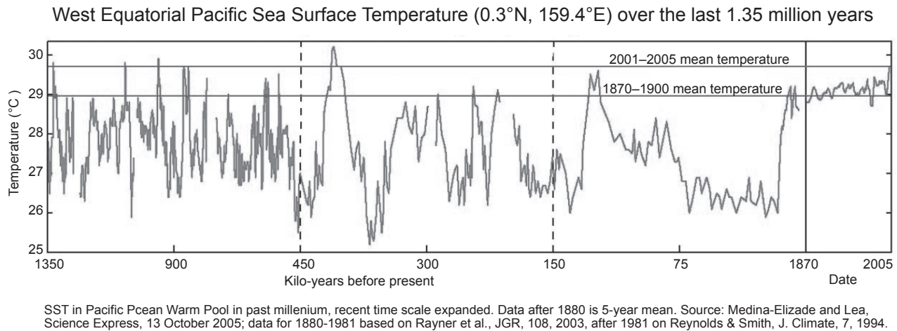
Figure 1: West equatorial Pacific sea surface temperature over the last 1.35 million years
