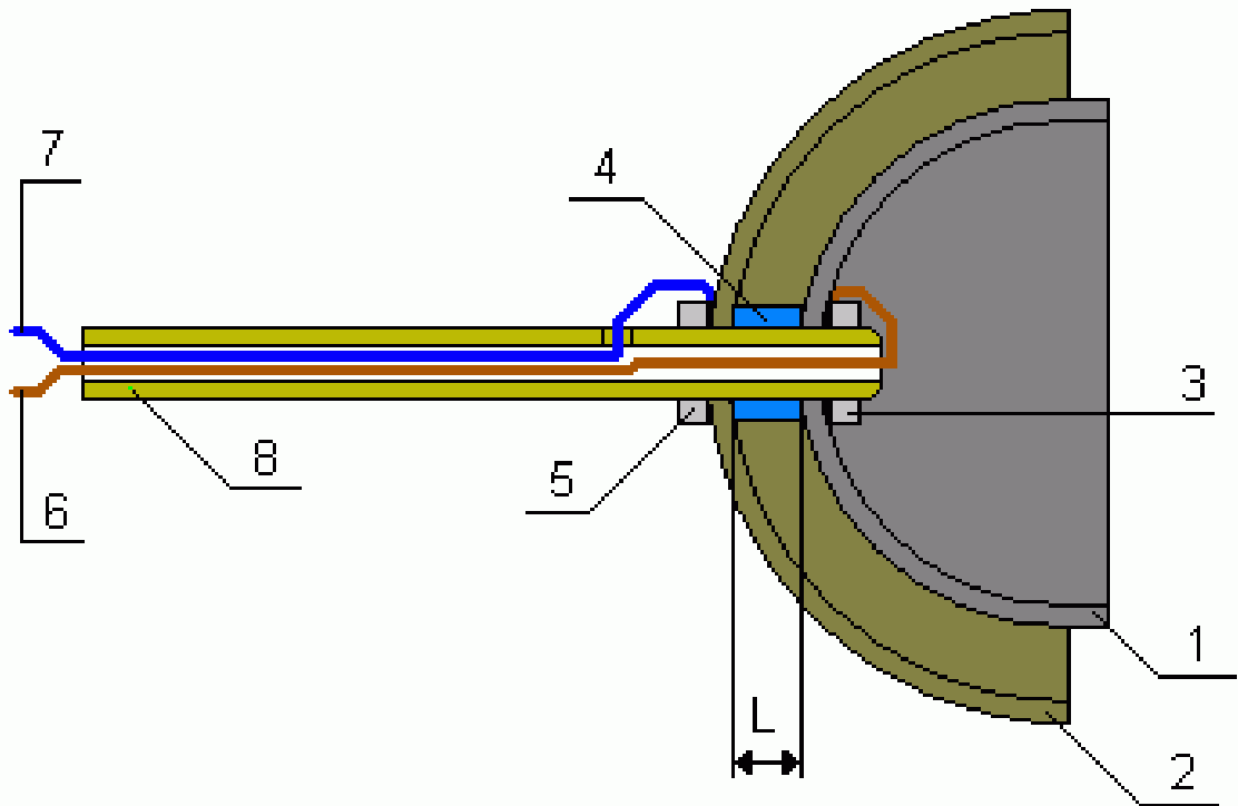
Fig. #E2: The above drawing illustrates the general design and main components of the telekinetic heater of Mr Davey. Notice that it can easily be enlarged by clicking onto it. Descriptions of subsequent components of this heater are provided in subsection LA3.3 from volume 10 of monograph [1/5] . (The above illustration originates from monograph [1/5] where it is shown as part (3) on Figure LA8 - courtesy "szod".)
